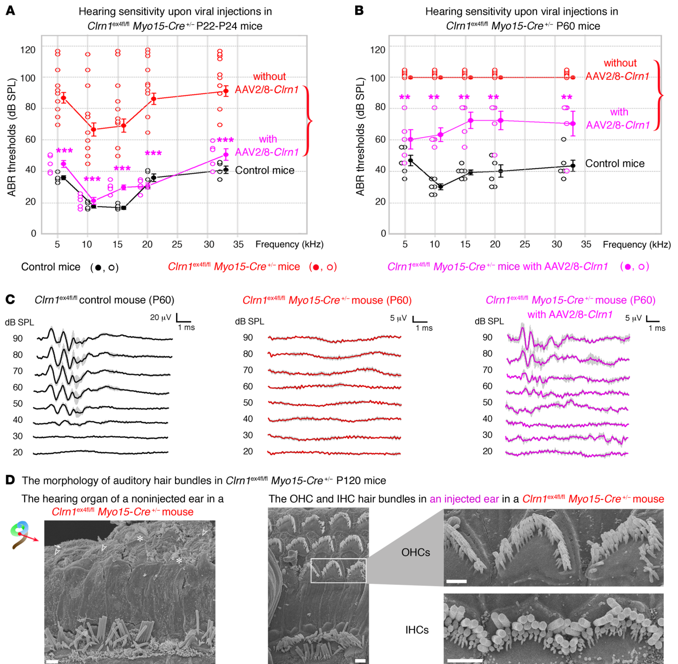
Figure 9. AAV2/8-mediated delivery of clarin-1 in Clnr1 ex4fl/fl Myo15-Cre +/- mice leads to long-term preservation of hearing. (A) Comparative tone-burst ABR thresholds (audiogram, mean \pm SEM and individual points for each frequency) in AAV2/8- Clnr1 -injected (purple, n = 7 ) and untreated (red, n = 10 ) inner ears of P22-P24 Clnr1 ex4fl/fl Myo15-Cre +/- mice and control (black, n = 6 ) mice. (B) Similar comparative audiograms for AAV2/8- Clnr1 -injected (purple, n = 5 ) and untreated (red, n = 6 ) inner ears of P60 Clnr1 ex4fl/fl Myo15-Cre +/- mice and P60 control (black, n = 6 ) mice. (C) Mean click ABR waves at P60 in control and in untreated and AAV2/8- Clnr1 -injected Clnr1 ex4fl/fl Myo15-Cre +/- mice. (D) Scanning electron microscopy view of stereocilia from untreated (left) and AAV2/8- Clnr1 -injected (right) ears of P120 Clnr1 ex4fl/fl Myo15-Cre +/- mice ( n = 3 ). By contrast to the untreated ears, the injection of AAV2/8- Clnr1 resulted in apparently normal hair bundles still visible on P120 ( n = 3 ). However, despite the persistence of V-shaped bundles, the stereocilia in the short and middle rows are heterogeneous in length, and many of these stereocilia are missing. ** P < 0.01 , *** P < 0.001 (unpaired Student's t test). Scale bars: 1 \mu m.
