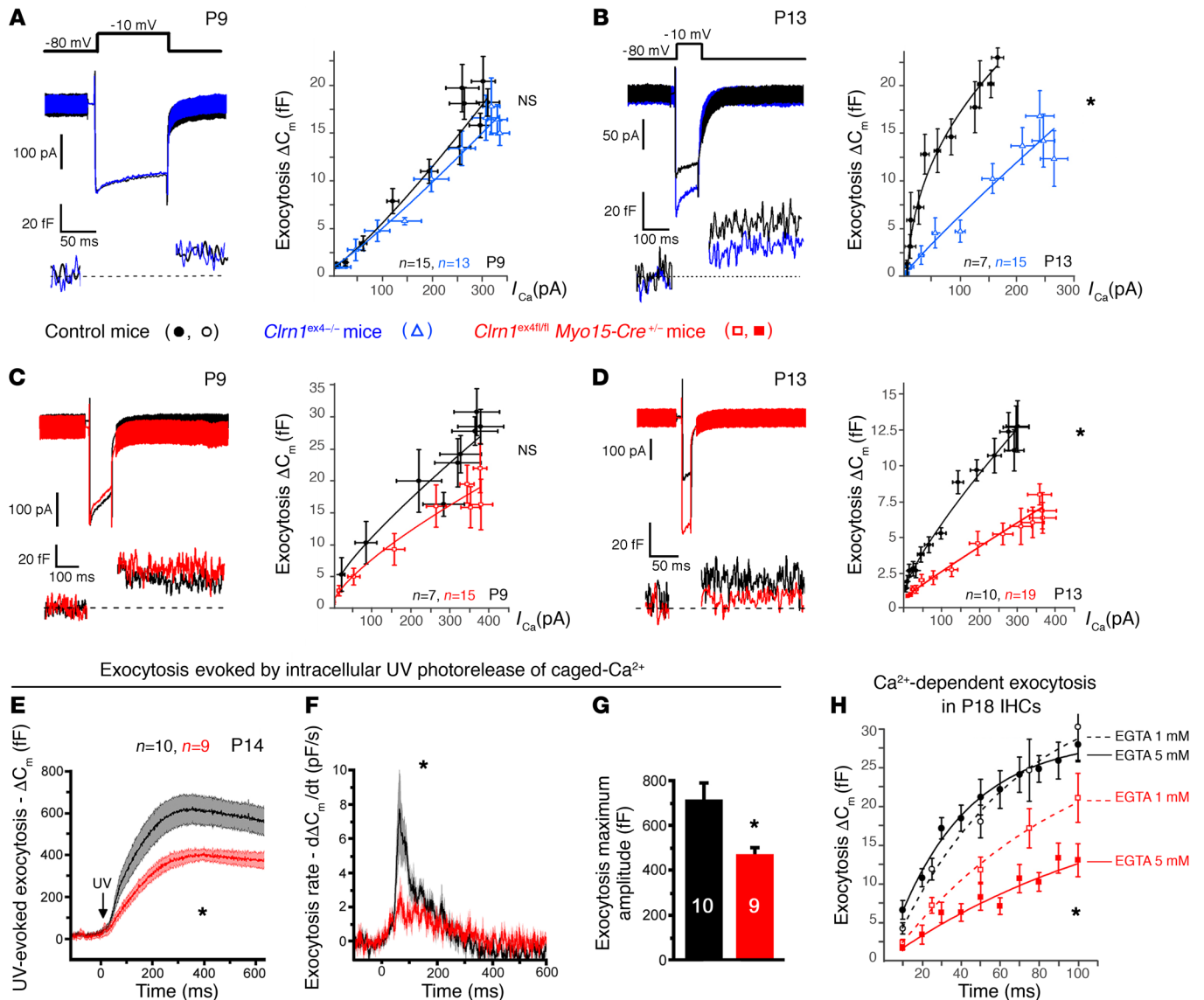
Figure 5. Ca^{2+} -mediated exocytosis in mutant IHCs lacking clarin-1. (A–D) Exocytosis was measured after various voltage steps between -80 mV and -5 mV, with each voltage step lasting 100 milliseconds (A–C) or 25 milliseconds (D). A simple power function was fitted to the data ( y = ax^N , where a is exocytosis slope efficiency and N the power index; Supplemental Table 2). Ca^{2+} efficiency for IHC exocytosis was normal at P9, but was significantly lower in P13 Clrn1 ex4/- mice ( a = 0.04 \pm 0.01 fF/pA) than in control littermates ( a = 0.16 \pm 0.01 fF/pA; P < 0.05 ) and in P13 Clrn1 ex4fl/fl Myo15-Cre +/- mice ( a = 0.07 \pm 0.01 fF/pA) than in control littermates ( a = 0.16 \pm 0.01 fF/pA; P < 0.05 ). (E–G) Mean exocytotic response curves evoked by UV uncaging of intracellular Ca^{2+} in IHCs from P14 Clrn1 ex4fl/fl Myo15-Cre +/- (red) and control (black) mice. (F) Exocytosis rates obtained by a derivative function ( dC_m/dt ) of the curves shown in E. (G) Comparative exocytotic peak upon Ca^{2+} photorelease in mutant and control IHCs. (H) Exocytosis kinetics for constant voltage steps from -80 to -10 mV, with durations increasing from 10 to 100 milliseconds, in IHCs from P18 Clrn1 ex4fl/fl Myo15-Cre +/- (red) and control (black) mice. The intracellular Ca^{2+} buffer was 1 mM or 5 mM EGTA. A simple exponential function was fitted to the data, with similar time constants of 25 \pm 10 milliseconds ( n = 12 ) and 33 \pm 18 milliseconds ( n = 11 ) for controls in 1 mM and 5 mM EGTA, respectively. For Clrn1 ex4fl/fl Myo15-Cre +/- IHCs, the time constant increased from 102 \pm 50 milliseconds ( n = 27 ) in 1 mM EGTA to 205 \pm 32 milliseconds ( n = 10 ) in 5 mM EGTA ( P < 0.05 ). The values shown are means \pm SEM; * P < 0.05 (A–F and H, 2-way ANOVA; and G, Mann-Whitney test).
