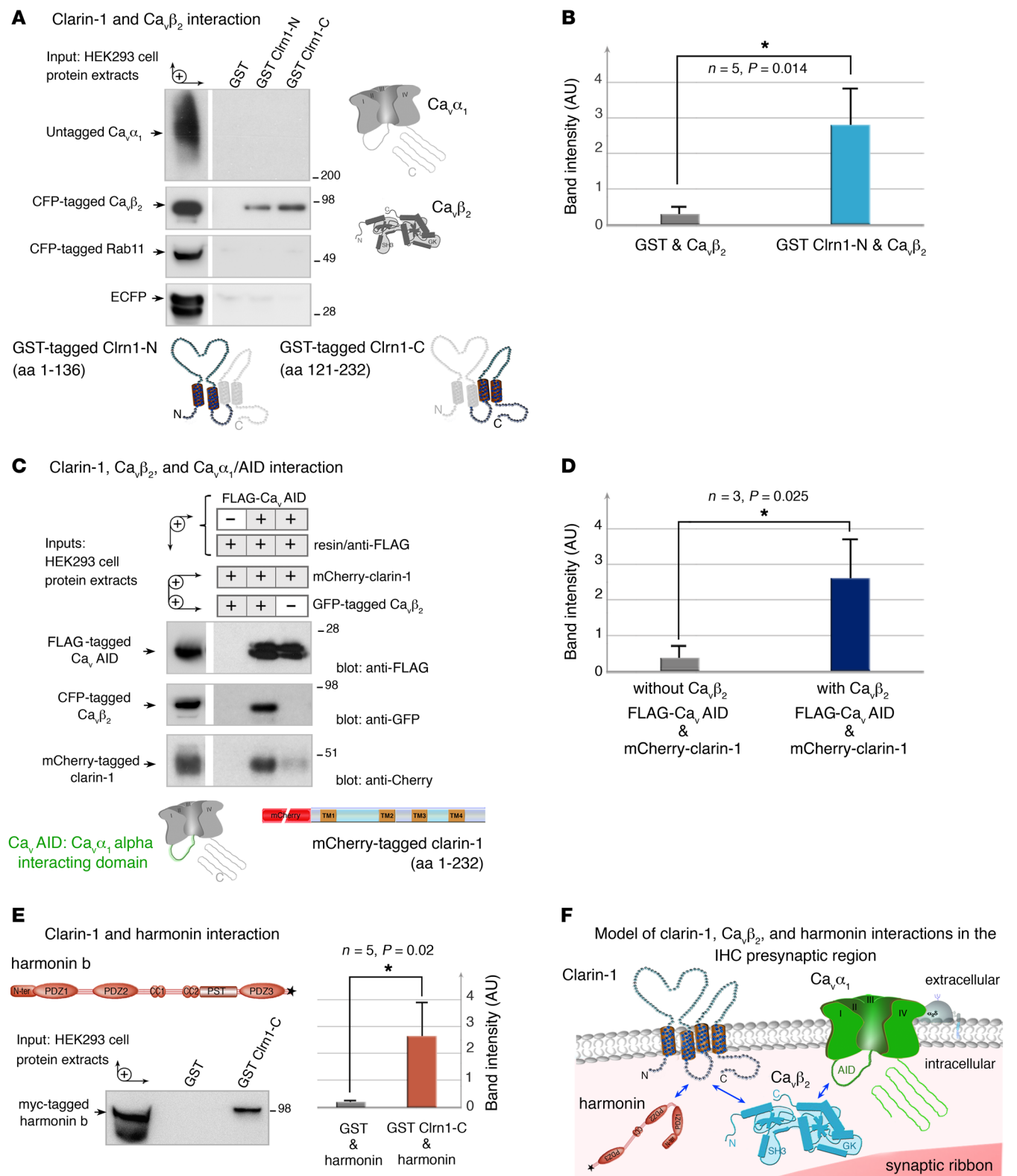
Figure 11. Interactions between clarin-1, the Ca_v1.3 channel complex, and harmonin. (A and B) The GST-tagged clarin-1 N-terminal region (Clrn1-N) and C-terminal region (Clrn1-C) bind to CFP-tagged Ca_v\beta_2 produced in HEK293 cells, whereas GST alone does not. No binding is detected with the untagged Ca_v\alpha_1 , CFP-tagged Rab11, or ECFP alone. (B) The bar chart indicates the significant interaction between clarin-1 and Ca_v\beta_2 ( n = 5, *P < 0.05 ; unpaired Student's t test). (C and D) In a coimmunoprecipitation assay, anti-FLAG M2 resin was incubated with HEK293 cells coproducing FLAG-tagged Ca_v AID, mCherry-tagged clarin-1, and CFP-tagged Ca_v\beta_2 , or mCherry-tagged clarin-1 and CFP-tagged Ca_v\beta_2 . (D) Significant binding between Ca_v AID and clarin-1 is observed only in the presence of Ca_v\beta_2 ( n = 3, *P < 0.05 ; unpaired Student's t test). (E) GST-tagged Clrn1-C binds to myc-tagged harmonin b, whereas GST alone does not. The bar chart shows the significant interaction between clarin-1 and harmonin ( n = 5, P < 0.05 ; unpaired Student's t test). (F) Schematic representation of a synaptic active zone summarizing the interactions between clarin-1, the Ca^{2+} channel subunits Ca_v\beta_2 and Ca_v\alpha_1 , and harmonin (see uncut gels in supplemental material).
