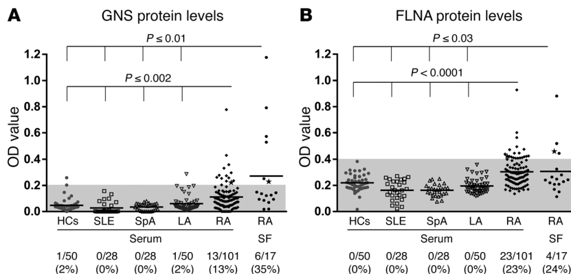
Figure 5. GNS and FLNA protein levels in RA patients and comparison group subjects. GNS and FLNA protein concentrations were measured in serum and SF samples from patients with RA, serum samples from patients with CTD, SpA, or LA, and serum samples from HCs. ( A ) GNS protein concentrations and ( B ) FLNA protein concentrations are shown, as measured by ELISA assay. For both analyses, positivity was defined as greater than 3 SD above the mean value for HC subjects (area above the shaded region). Symbols represent values for individual patients, and horizontal lines indicate the mean values. The values for patient RA1 are indicated with a star. Only significant P values, determined by unpaired, 2-tailed t test with Welch's correction, are shown. SLE, systemic lupus erythematosus.
