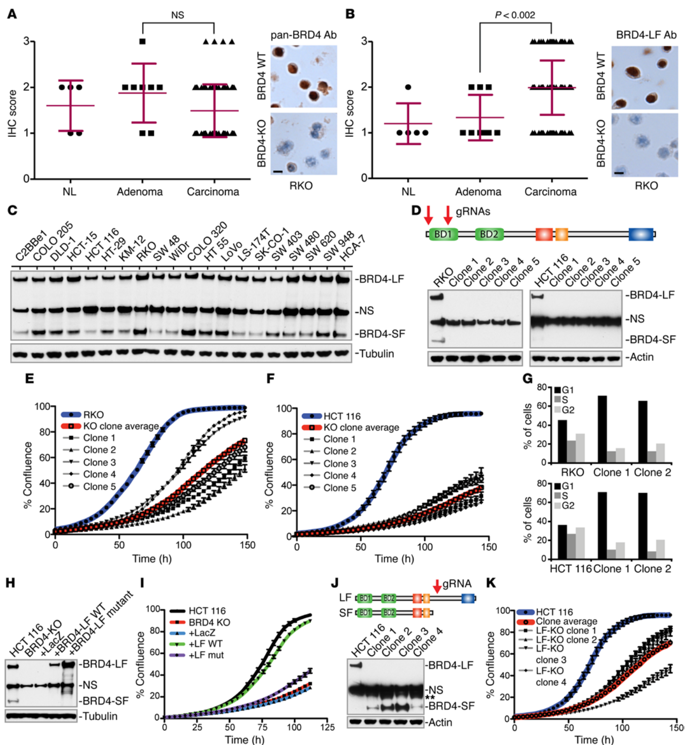
Figure 2. BRD4-LF is essential for colon cancer growth. (A and B) BRD4 IHC of normal colon (NL), colonic adenoma, and colonic carcinoma using either a pan-isoform BRD4 (A) or a BRD4-LF-specific (B) Ab. Photomicrographs illustrate target specificity using WT or BRD4-KO RKO cells. Data represent the mean \pm SD. Statistical comparisons in A and B were made using a 2-tailed Student's t test. Scale bars: 10 \mu m (A and B). (C) Immunoblot analysis of isoform-specific BRD4 expression in colon cancer cell lines. (D) Generation of clonal BRD4-KO RKO and HCT 116 cells. Schematic illustrates the location of the gRNAs. Immunoblot analysis of multiple BRD4-KO clones is shown. (E and F) IncuCyte analysis was used to quantify cell proliferation of RKO (E) and HCT 116 (F) BRD4-KO cells. Blue line represents parental cells; gray lines represent an individual clone's growth; and red line represents average clonal growth. Error bars represent the SEM. (G) FACS-based cell-cycle analysis of RKO and HCT 116 parental and BRD4-KO cells. (H and I) Expression of the BRD4-LF-rescued (LF WT) cell proliferation defects in HCT 116 BRD4-KO cells. Expression of LacZ or a BRD4-LF containing inactivating mutations in both bromodomains (LF mut) failed to rescue the phenotype. (H) Immunoblot of stably expressing cell lines in I. (J and K) Generation of clonal HCT 116 cells that lacked the C-terminal domain of BRD4. (J) Schematic illustrates the location of the gRNA. Immunoblot highlights 4 resulting BRD4 clones with deleted C-termini. BRD4-LF truncated products are highlighted by a double asterisk. (K) IncuCyte analysis was used to quantify cell proliferation of HCT 116 cells containing BRD4 C-terminal deletions. Blue line represents parental cells; gray lines represent an individual clone's growth; and red line represents average clonal growth. Error bars represent the SEM.
