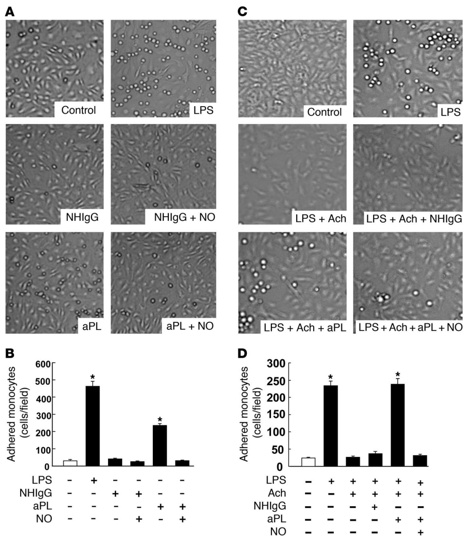
Figure 1 aPL-mediated increases in monocyte adhesion are due to decreased bioavailable NO. (A) Monocyte adhesion to BAECs was evaluated under the following conditions: untreated control, LPS (100 ng/ml), NHIgG (100 μg/ml), NHIgG + NO donor (SNAP, 20 μmol/l), aPL (100 μg/ml), and aPL + NO donor. (B) Graph representing summary data for A. (C) Monocyte adhesion to BAECs was evaluated under the following conditions: untreated control, LPS, LPS + Ach (10 μmol/k), LPS + Ach + NHIgG, LPS + Ach + aPL, and LPS + Ach + aPL + NO donor SNAP. (D) Graph representing summary data for C. In B and D, n = 4; *P < 0.05 versus control. Original magnification, ×40 (A and C).
