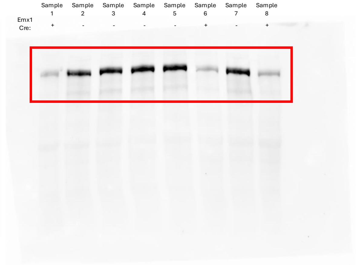
Immunoblot: USP15
