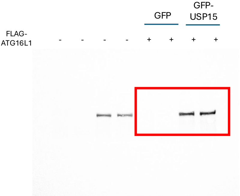
Immunoblot: GFP
