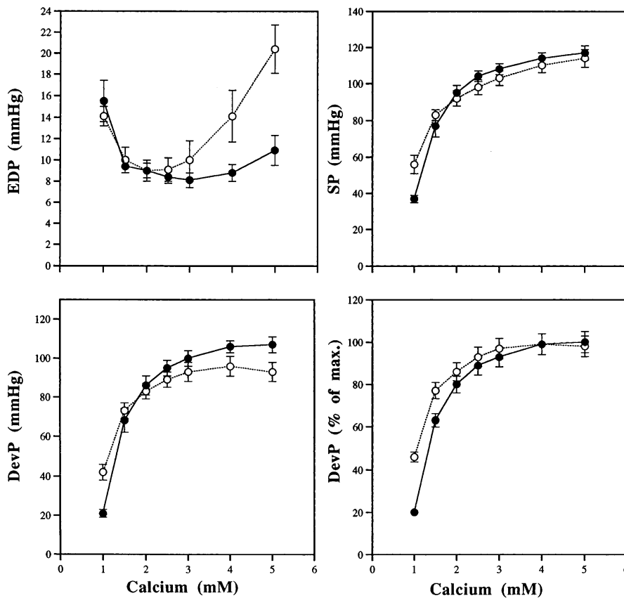
Figure 2. Relationships between perfusate calcium concentration and parameters of left ventricular function in wild-type (filled circles) and \alpha MHC 403/+ (open circles) hearts. \alpha MHC 403/+ hearts generated more left ventricular pressure than wild types at 1 mM Ca 2+ , but had a lower maximal DevP due to an increased EDP. When DevP was normalized as a percentage of maximal DevP, there is a leftward shift in the calcium dose-response relationship in \alpha MHC 403/+ hearts, suggesting increased calcium sensitivity at low Ca 2+ concentrations.
