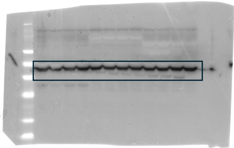
IB: Beta-Actin
