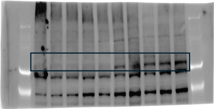
IB: FAM20C
