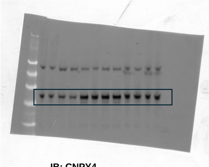
IB: CNPY4
