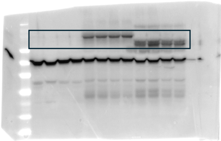
IB: FAM20C
