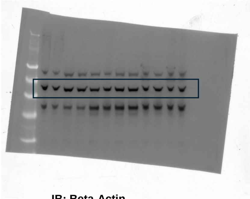
IB: Beta-Actin
