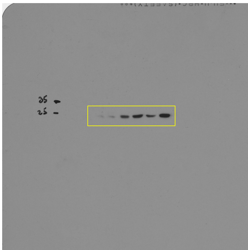
Anti-FTL1
