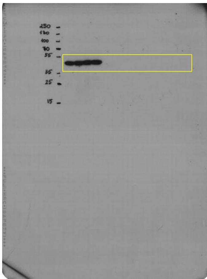
Anti-actin
