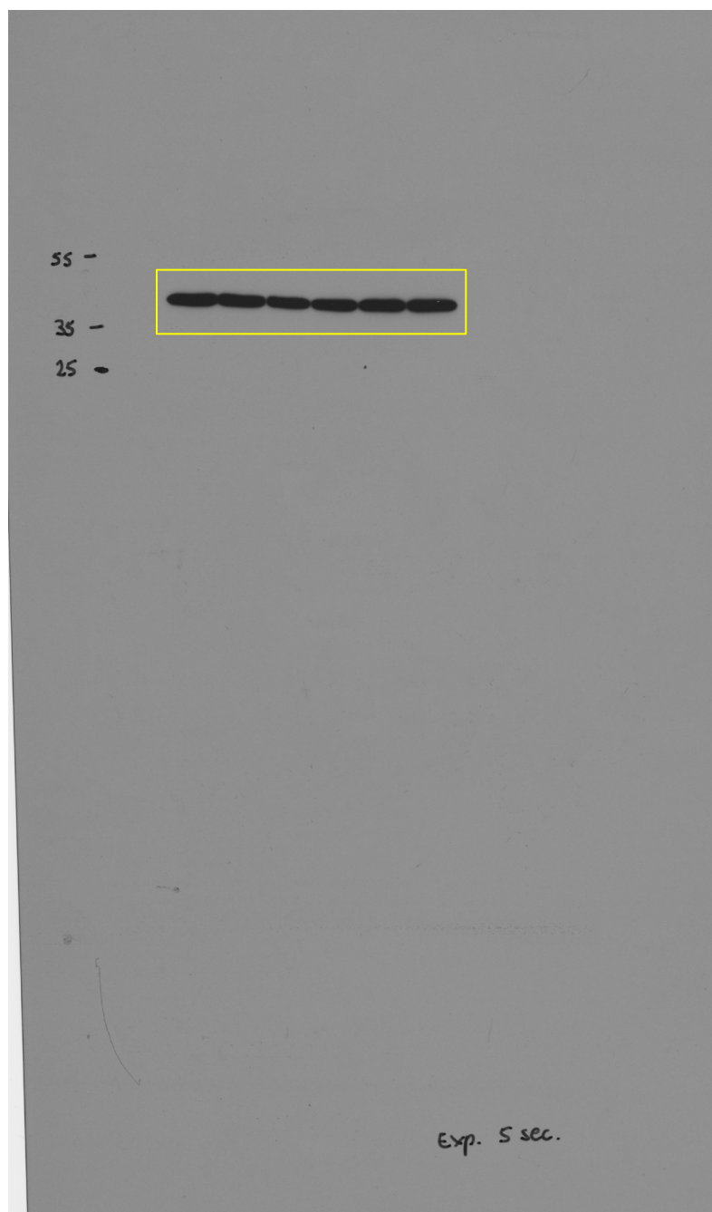
Anti-actin
