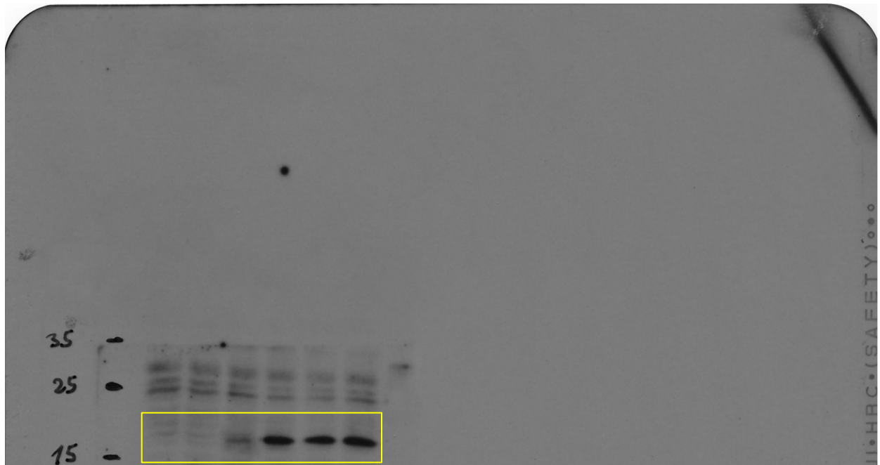
Anti-FTL1
