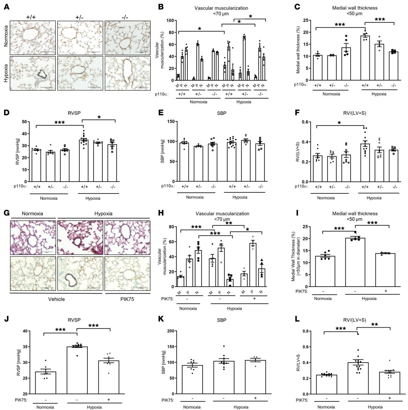
Figure 5. SM-specific p110 \alpha deficiency and pharmacological inhibition of p110 \alpha prevent hypoxia-induced pulmonary hypertension. (A) Representative immunostainings of small pulmonary arteries from sm-p110 \alpha^{+/+} , sm-p110 \alpha^{+/-} , and sm-p110 \alpha^{-/-} mice exposed to normoxia or hypoxia (10% O 2 for 21 days). Shown are representative images of lung sections immunostained for vWF (brown) and \alpha -smooth muscle actin (purple), 400-fold magnification. Scale bar: 100 \mu m. (B) Quantitative morphometric analysis of muscularization of small (<70 \mu m) pulmonary vessels from the above animals. Shown is the percentage of fully (M), partially (P), and nonmuscularized (N) vessels (at least 80 analyzed per animal), n = 5, 4, 5, 5, 5, 5. (C) Quantitative assessment of medial wall thickness of small (<50 \mu m) pulmonary arteries from the above animals (n = 5, 4, 5, 5, 4, 5). (D) RVSP (mmHg), measured by a Millar microtip catheter (1F) inserted into the right ventricle via the jugular vein, n = 8, 7, 8, 14, 8, 7. (E) SBP (mmHg) was measured using a Millar microtip catheter (1F) inserted into the left carotid artery, n = 8, 6, 8, 14, 8, 6. (F) RV hypertrophy is shown as RV/LV + S ratio, n = 8, 7, 8, 12, 8, 5. (G-L) Pulmonary vascular remodeling and pulmonary hemodynamics of PIK75-treated WT mice exposed to hypoxia. (G) Representative images of Van Gieson staining demonstrating the medial wall thickness (upper panel) and double-immunostaining for vWF and \alpha -smooth muscle actin demonstrating the muscularization (lower panel) of peripheral pulmonary arteries. Scale bar: 100 \mu m. (H) Impact of p110 \alpha inhibition with PIK75 on vascular muscularization of small (<70 \mu m) pulmonary arteries, n = 6, 5, 4 and (I) medial wall thickness of less than 50 \mu m pulmonary arteries, n = 6, 5, 4. (J) Impact of p110 \alpha inhibition with PIK75 on RVSP, n = 7, 10, 8; (K) SBP, n = 7, 9, 5, and (L) RV hypertrophy, expressed as the RV/LV + S ratio; n = 12, 14, 11. All data represent mean \pm SEM. *P < 0.05; **P < 0.01; ***P < 0.001 as assessed by ANOVA followed by a Newman-Keuls post hoc test.
