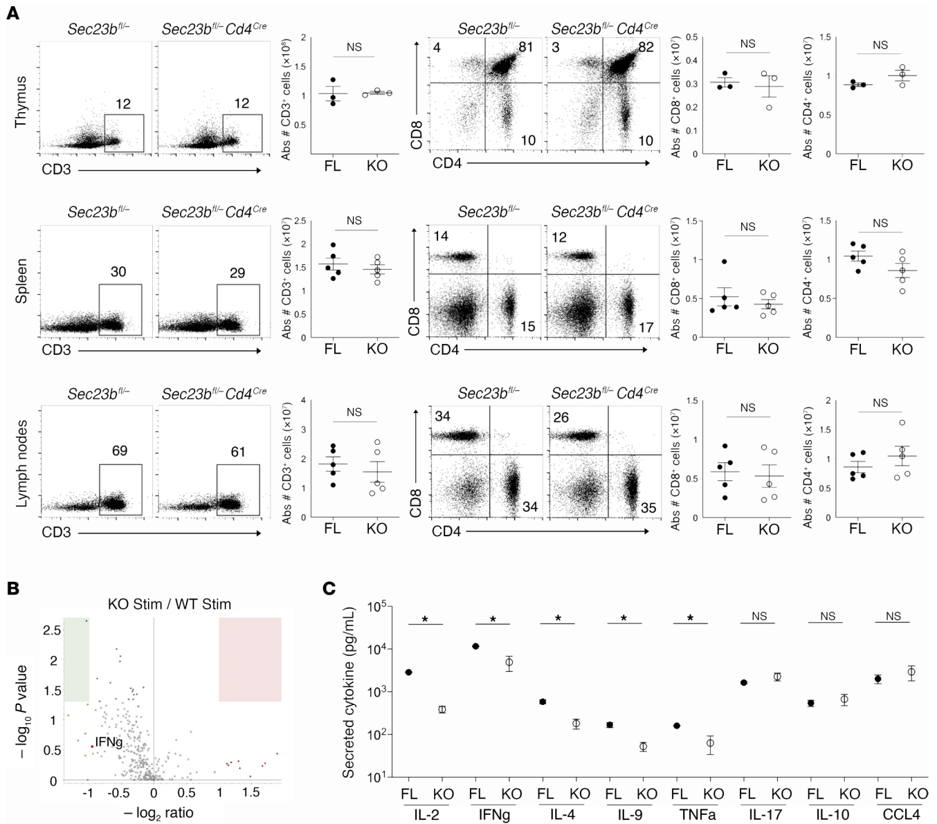
Figure 2. SEC23B deficiency does not affect mature T cell development but regulates its secretome. (A) Percentages and absolute numbers of Sec23b fl/- (FL) and Sec23b fl/- Cd4 Cre (KO) CD3 + T cells in whole thymus ( n = 3 ), spleen ( n = 5 ), and lymph node ( n = 5 ) homogenate samples (left), and those of CD4 + and CD8 + T cell subsets gated on CD3 + cells (right). (B) Volcano plot representing 3 biological replicates of SEC23B-deficient T cell secretomes after 24 hours of stimulation compared with WT. Log 2 ratios were calculated based on P values. (C) Luminex panel showing mean cytokine levels derived from Sec23b fl/- (FL) and Sec23b fl/- Cd4 Cre (KO) T cell supernatants following 3 days of stimulation with \alpha CD3 and \alpha CD28. (A and C) Data represent mean \pm SEM, with * P < 0.05 (2-tailed unpaired Student's t test).
