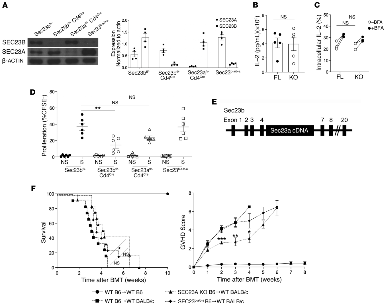
Figure 5. Mechanisms of COPII-dependent regulation of T cell functions. (A) Representative Western blot showing SEC23B and SEC23A expression in purified T cells from Sec23b fl/- , Sec23b fl/- Cd4 Cre , Sec23a fl/- Cd4 Cre , and Sec23 b-a/b-a mice. Normalized levels of each protein relative to \beta -actin are plotted on the right ( n = 4 /group). (B) ELISA measuring IL-2 secreted by WT and SEC23A-deficient T cells over 3 days in culture with \alpha CD3- and \alpha CD28-stimulating antibodies ( n = 5 /group). (C) Flow cytometry measuring levels of intracellular IL-2 in WT and SEC23A-deficient T cells following their stimulation in vitro for 3 days with \alpha CD3 and \alpha CD28, and 5 hours with PMA and ionomycin in the presence or absence of BFA ( n = 3 /group). (D) Proliferation of isolated T cells from the indicated mice stimulated in vitro with \alpha CD3 and \alpha CD28, as measured by CFSE dilutions ( n = 6 /group). (E) Schematic diagram of Sec23b endogenous genomic locus in Sec23 b-a/b-a mice, which contains the Sec23a coding sequence (from C367 to A2298) followed by a poly(A) termination signal in lieu of the full Sec23b sequence as previously described (26). (F) Survival and composite GVHD scores of mice ( n = 12 /group) that received syngeneic T cell-depleted bone marrow and T cells from either syngeneic WT C57BL/6J donors or allogeneic WT C57BL/6J, Sec23a fl/- Cd4 Cre C57BL/6J, or Sec23 b-a/b-a C57BL/6J donors. (B and C) Significance was determined by 2-tailed unpaired Student's t test. (D) Significance was determined by 1-way ANOVA and post hoc Tukey's tests; ** P < 0.01 . (F) Significance was determined by Mantel-Cox log rank test for survival and 1-way ANOVA and post hoc Tukey's tests for GVHD score; * P < 0.05 , ** P < 0.01 , *** P < 0.001 .
