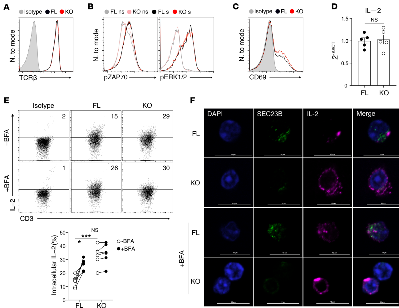
Figure 3. Deficiency of SEC23B-dependent COPII leads to accumulation of secreted proteins. (A) Histograms based on flow cytometry of surface TCR-β on Sec23b fl/- and Sec23b fl/- Cd4 Cre T cells relative to isotype levels present on naive unstimulated WT T cells. (B) Flow cytometry of phosphorylated ZAP70 and ERK1/2 molecules in Sec23b fl/- and Sec23b fl/- Cd4 Cre T cells that received no stimulation or stimulation with αCD3 and αCD28 for 30 minutes. (C) Flow cytometry of surface CD69 present on Sec23b fl/- and Sec23b fl/- Cd4 Cre T cells stimulated with αCD3 and αCD28 for 6 h compared with isotype levels present on naive unstimulated WT T cells. Flow cytometric data are representative of 3 replicate experiments. (D) qRT-PCR analysis of IL-2 in SEC23B-deficient T cells compared with WT following stimulation with αCD3 and αCD28 for 4 days ( n = 5 /group). (E) Flow cytometry measuring intracellular IL-2 levels in T cells after stimulation by αCD3 and αCD28 for 3 days followed by 5 hours of stimulation with PMA and ionomycin in the presence or absence of BFA ( n = 6 /group). (F) Immunofluorescence confocal micrographs of SEC23B (green) and IL-2 (pink) in WT or SEC23B-deficient T cells after 3 days of αCD3 and αCD28 stimulation, and 5 hours of PMA and ionomycin stimulation with or without BFA. (D) Data represent mean ± SEM, and significance was determined by 2-tailed unpaired Student's t test. (E) Statistical significance was determined by 1-way ANOVA and post hoc Tukey's test; * P < 0.05 , *** P < 0.001 . Scale bars: 10 μm.
