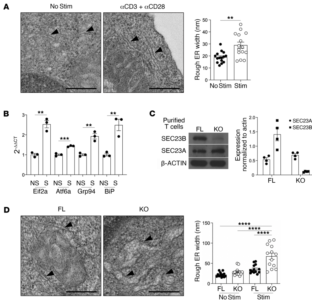
Figure 1. COPII-dependent ER-to-Golgi pathway is engaged upon T cell activation. (A) Transmission electron micrographs of WT murine T cells that received no stimulation or stimulation with \alpha CD3 and \alpha CD28 for 3 days. Measurements of rough ER widths were taken from 3 different ERs from 5 cells in each group ( n = 15 ). Scale bars: 100 nm. (B) Real-time quantitative PCR analysis of ER stress-associated genes in WT murine T cells that received no stimulation or 24 hours of stimulation with \alpha CD3 and \alpha CD28 ( n = 3 ). (C) Western blots showing protein levels of SEC23B, SEC23A, and \beta -actin in Sec23b fl/- Cd4 Cre (KO) T cells relative to Sec23b fl/- (FL) controls. Densitometric analysis on the right plot indicates normalized levels of SEC23A and SEC23B relative to \beta -actin expression ( n = 4 ). (D) TEM highlighting an increase in rough ER dilation in Sec23b fl/- Cd4 Cre T cells when compared with Sec23b fl/- controls following activation with \alpha CD3 and \alpha CD28 for 3 days ( n = 13 ). Scale bars: 100 nm. (A and B) Data represent mean \pm SEM, with ** P < 0.01 and *** P < 0.001 (2-tailed unpaired Student's t test). (D) Statistical significance was determined by 1-way ANOVA and post hoc Tukey's test; **** P < 0.0001 .
