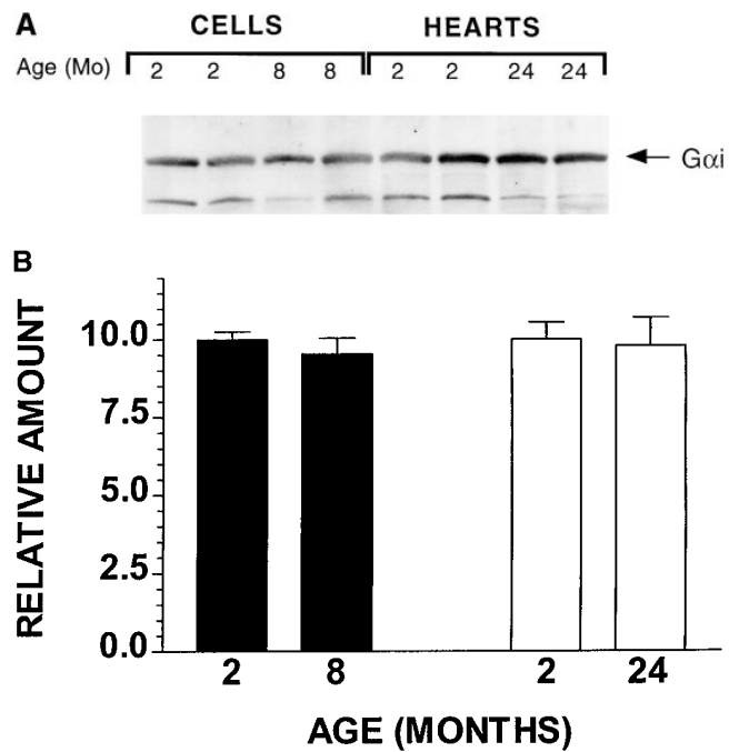
Figure 3. Abundance of G \alpha_i . (A) Representative protein immunoblot for G \alpha_i in membranes purified from isolated ventricular myocytes (2 and 8 mo) or heart tissue (2 and 24 mo). Duplicate samples of 40 \mu g of membrane protein were electrophoresed and transferred to nitrocellulose as described in Methods. A commercially available polyclonal antiserum was used (G \alpha_{i(1-3)} , Santa Cruz Biotechnology) and the major immunoreactive band detected by standard chemiluminescence migrated at the expected size of G \alpha_i (arrow, ~43 kD). (B) Histogram showing the mean + SEM of laser densitometry scans of four immunoblots from four individual hearts (open bars) or cell preparations (solid bars) of each age done in duplicate.
