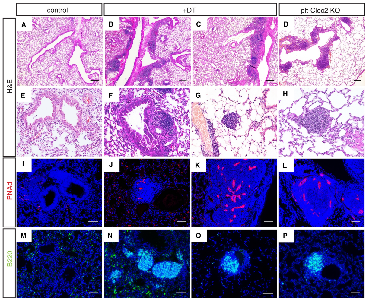
Figure 7: TLOs after lung lymphatic ablation resemble those in plt-Clec2 KO mice. (A-H) H&E staining of lung tissue from control transplanted lungs, DT-treated iDTR;VEGFR3Cre ERT2 transplanted lungs with lymphatic ablation, and lungs from plt-Clec2 KO mice. (I-P) Immunohistochemistry for B cells (B220, green) and HEVs (PNAd, red) in control transplanted lungs, DT-treated iDTR;VEGFR3Cre ERT2 transplanted lungs, and plt-Clec2 KO lungs. Data representative of 4 mice in each group. Scale bars in A-D = 100µm. All other scale bars = 25µm.
