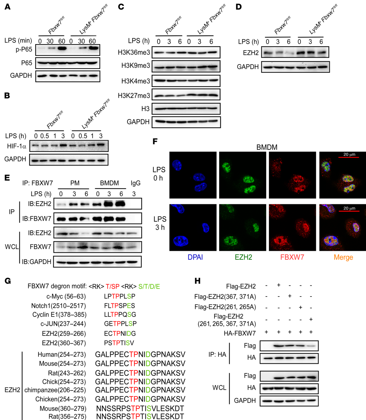
Figure 6. FBXW7 interacts with EZH2. Immunoblot analysis of phosphorylated P65 (p-P65) and total P65 ( A ), HIF-1 \alpha ( B ), H3 histone modification ( C ), and histone methyltransferase EZH2 protein levels ( D ) in lysates of BMDMs from Fbxw7 fl/fl and LysM + Fbxw7 fl/fl mice stimulated with LPS for the indicated durations. ( E ) Coimmunoprecipitation (IP) and immunoblot (IB) of BMDMs stimulated with LPS for the indicated durations. ( F ) Confocal microscopic imaging of BMDMs that were stimulated with LPS and labeled with Abs against the appropriate protein. ( G ) Sequence alignment of EZH2 with FBXW7 degron motif (<RK>S/TP<RK>XS/T/E/D), where X and <RK> are any amino acid, except arginine (R) or lysine (K). ( H ) Coimmunoprecipitation and immunoblot analysis of HEK293T cells transfected with HA-FBXW7 along with a vector for Flag-EZH2 (WT), Flag-EZH2 (261 and 265A), Flag-EZH2 (367 and 371A), and Flag-EZH2 (261 and 265, 367, and 371A, 4A). and treated with MG132, followed by immunoprecipitation with anti-HA-M2 beads. All data are representative of at least 3 independent experiments.
