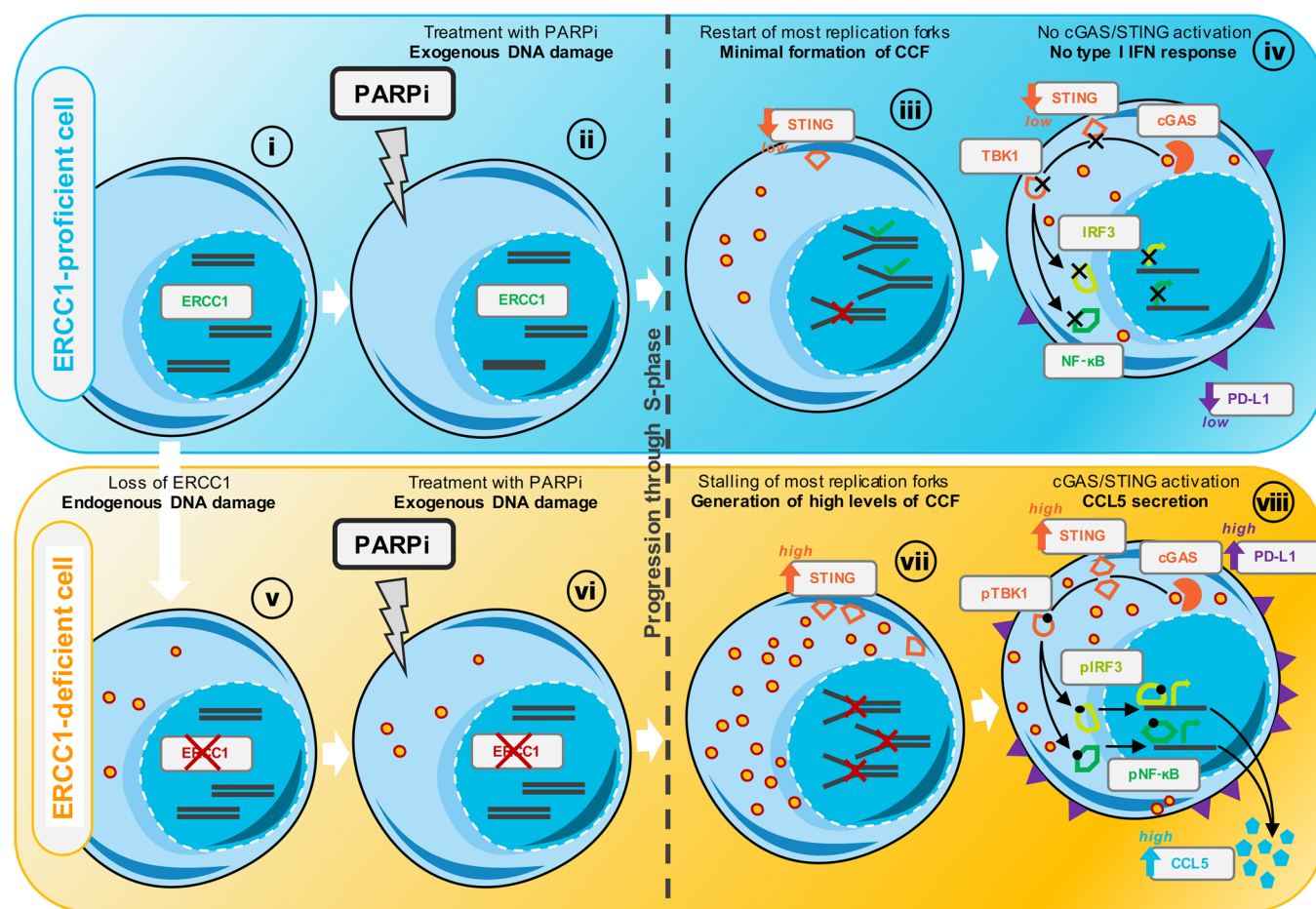
Figure 10. Model of ERCC1 defect-dependent activation of cGAS/STING following PARPi exposure. (i) ERCC1 WT/WT cells have a functional DDR and adequately maintain genome integrity. (ii) Upon PARPi exposure, exogenous DNA damage is triggered, mostly initiated by PARP1 itself trapped onto the DNA at sites of spontaneous single-strand breaks (SSBs). (iii) During the S phase of the cell cycle, trapped PARP1 generates lesions that prevent the progression of replication forks, leading to fork stalling and subsequent formation of DSBs. In ERCC1 WT/WT cells, most trapped PARP1 lesions are removed, which enables the processing of DSBs through HR and eventually allows replication to restart. Residual inadequately repaired lesions cause moderate formation of CCFs. (iv) The low levels of CCFs generated are unable to trigger the pTBK1/IRF3/NF-κB signaling cascade or subsequent transcription of type I IFN genes; PD-L1 is moderately induced. (v) ERCC1 -/- cells are exposed to increased endogenous DNA damage following the loss of ERCC1. This generates minimal levels of CCFs. (vi) Upon PARPi exposure, ERCC1 -/- cells are subjected to an additional exogenous source of DNA damage. (vii) During the S phase of the cell cycle, trapped PARP1 generates lesions that prevent the progression of replication forks, leading to stalling of forks and subsequent formation of DSBs. In the absence of ERCC1, trapped PARP1 lesions cannot be adequately resolved, which triggers increased DSBs and eventually generates high levels of CCFs. (viii) CCFs are detected by cGAS and, due to the enhanced expression of STING in ERCC1 -/- cells, these efficiently activate cGAS/STING signaling. Activated STING homodimer phosphorylates TBK1, which in turn phosphorylates IRF3 and NF-κB; this triggers their translocation into the nucleus and results in the transcription of type I IFN genes: CCL5 and other type I IFN cytokines are secreted. Higher PD-L1 expression is induced at the cell surface.
