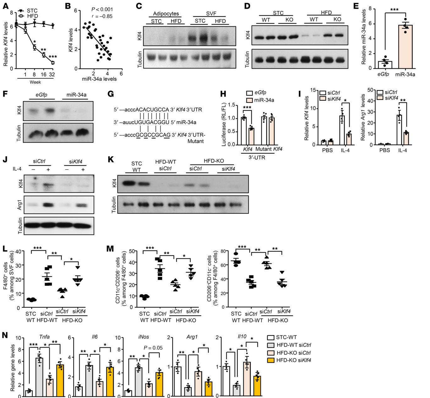
Figure 5. MiR-34a modulates inflammation and macrophage polarization by targeting Klf4 . (A) The mRNA abundance of Klf4 in epiWAT of mice ( n = 6-8 ). (B) Correlative analysis between the mRNA abundance of miR-34a and Klf4 levels ( n = 35 ). Correlation was assessed by nonparametric Spearman's test. (C) The protein levels of Klf4 in mature adipocytes and SVF of epiWAT isolated from mice on STC or HFD for 16 weeks. (D) Immunoblot analysis for Klf4 protein in SVF. (E and F) Analysis of miR-34a levels (E) and Klf4 protein levels (F) in bone marrow derived macrophages (BMDMs) infected with lentivirus encoding eGfp or miR-34a. ( n = 4 ). (G and H) A schematic diagram showing the construction of the luciferase reporter vectors (G), and luciferase assays were performed in HEK293 cells (H, n = 4 ). Data are presented as ratio of Renilla luciferase (RL) to firefly luciferase (FL) activity. (I and J) BMDMs were infected with lentivirus for 24 hours, followed by stimulation with IL-4 (10 ng/ml) for 24 hours. Analysis of gene expression of Klf4 and Arg1 (I) and protein levels of Klf4 and Arg1 (J) ( n = 4 ). (K-N) KO and WT littermates on HFD for 14 weeks were locally injected with lentivirus expressing siRNA against Klf4 ( siKlf4 ) or scramble control ( siCtrl ) in epiWAT for 2 weeks. (K) Immunoblot analysis for KLF4 protein in SVFs. (L and M) Flow cytometric quantification for percentage of total macrophages (L), M1 and M2 macrophages in SVFs (M, n = 4-5 ). (N) The mRNA abundance of M1 macrophage-associated genes in epiWAT ( n = 4-5 ). Data represent mean \pm SEM. Differences were determined by ANOVA (A, H, I, and L-N) or Student's t test (E); * P < 0.05 , ** P < 0.01 , *** P < 0.001 . MiR-34a abundance was normalized to sno202 level, and other gene levels were normalized to 18S RNA abundance.
