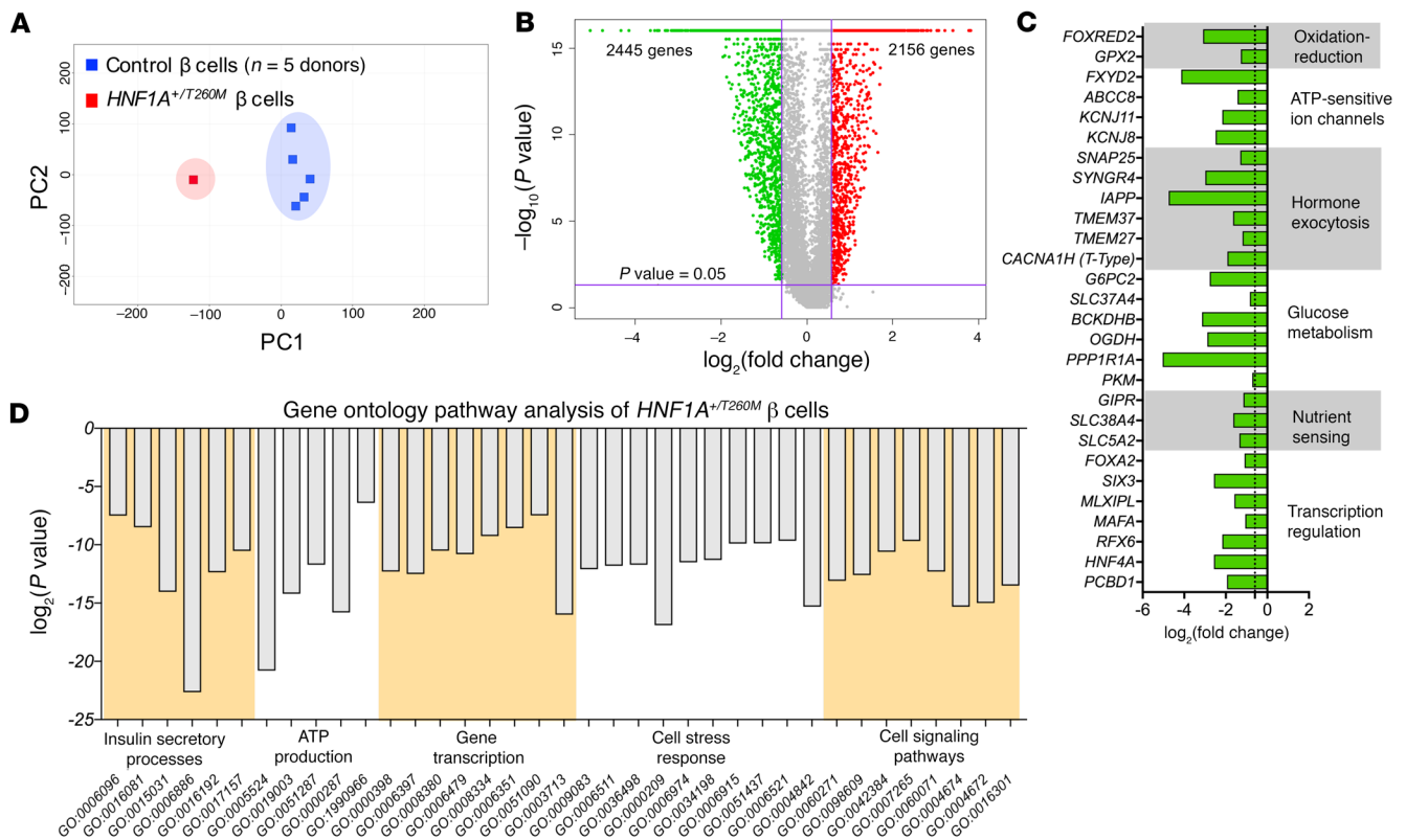
Figure 3. Transcriptomic analysis of HNF1A^{+/T260M} \beta cells. (A) Principal component analysis (PCA) plot depicts clustering of control \beta cells ( n = 5 donors; ages 26–55 years) (31) separate from HNF1A^{+/T260M} \beta cells. (B) The volcano plot demonstrates transcripts differentially expressed between control and HNF1A^{+/T260M} \beta cells (red, upregulated gene expression; green, downregulated gene expression). Differential expression was calculated based on fold change (FC) \geq 1.5 with a P -value cutoff of < 0.05 for calculated Z score. (C) Genes of interest and HNF1A targets are significantly downregulated in HNF1A^{+/T260M} \beta cells. The vertical dotted line represents FC = 1.5 times the threshold; P < 0.05 for all values shown. (D) Significant processes identified by Gene Ontology (GO) term-enrichment analysis are grouped and displayed by their P value on a \log_2 scale.
