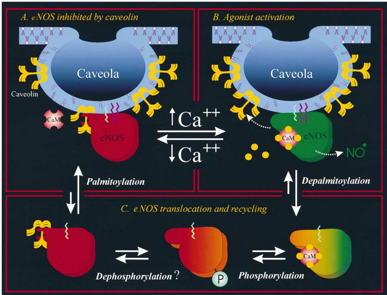
Figure 1. The cycle of eNOS activation and deactivation: reciprocal roles of \text{Ca}^{2+} -calmodulin and caveolin. (A) eNOS inhibited by caveolin. The interaction between eNOS and caveolin markedly attenuates enzyme activity in the resting endothelial cell. Shown is a plasmalemmal caveola characterized by its distinctive lipid content (cholesterol and glycosphingolipids vs. phospholipids in the adjacent noncaveolar plasma membrane) and by the presence of homo-oligomers of the membrane-associated scaffolding protein caveolin. The interaction of eNOS with the scaffolding domain of caveolin maintains the enzyme in its inactivated state (red). eNOS is shown as being dually acylated by N -myristoylation (teal) and by two molecules of palmitate (purple). The calcium regulatory protein calmodulin ( CaM ), which is enriched in the caveolar fraction of plasma membranes, does not bind to eNOS in the absence of \text{Ca}^{2+} . (B) Agonist activation. After agonist stimulation or other stimuli evoking a local increase in the [\text{Ca}^{2+}]_i concentration, \text{Ca}^{2+} -bound CaM competitively displaces caveolin from eNOS, thereby allowing the conformational changes within eNOS required for the electron transfer between the heme protein and reductase domains (not shown), leading to the synthesis of NO by the activated enzyme (green). The binding sites for \text{Ca}^{2+} - CaM and caveolin on eNOS appear to be located in the \text{NH}_2 -terminal domain of eNOS, and their binding is mutually exclusive. (C) eNOS translocation and recycling. The decline in [\text{Ca}^{2+}]_i seen after prolonged agonist activation leads to the dissociation of calmodulin from eNOS and deactivation of the enzyme as caveolin rebinds to eNOS. Caveats concerning the molecular details, subcellular locale, and temporal sequence of this speculative pathway are discussed in the text. In the model proposed here, prolonged agonist activation leads to eNOS depalmitoylation, translocation, phosphorylation, and, subsequently, to the rebinding of caveolin as the enzyme becomes dephosphorylated and repalmitoylated on its return to caveolae. eNOS remains myristoylated throughout; this modification probably guides the retargeting of the caveolin–eNOS complex to caveolae. Illustration by Naba Bora, Medical College of Georgia.
