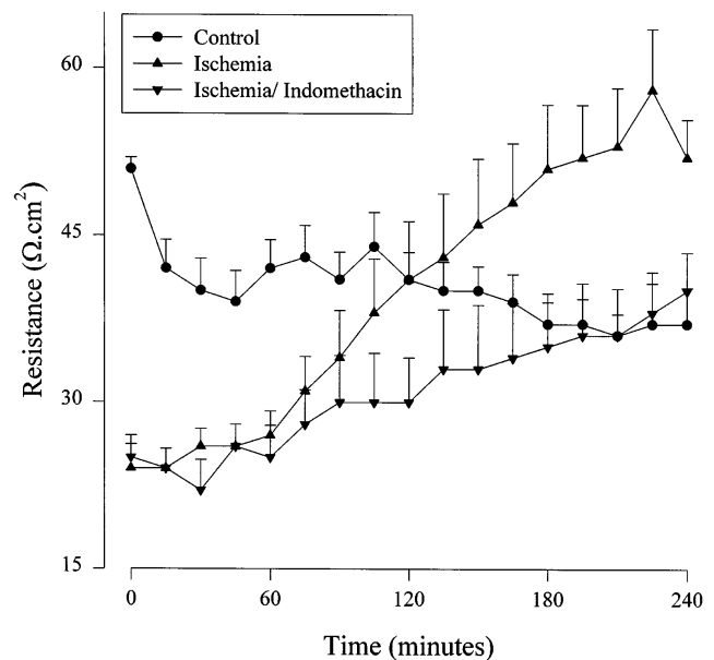
Figure 1. Electrical responses of repairing tissues. Tissues subjected to 1 h of ischemia had markedly reduced resistances at the beginning of the experiment. Control levels of resistance were attained in these tissues after 120 min, after which resistance continued to climb until it was approximately twofold that of control tissue. Addition of indomethacin to mucosal and serosal bathing solutions of injured tissues resulted in slower recovery of resistance, such that resistance only attained control levels of resistance at 240 min. Data points represent the mean \pm SE, n = 6 .
