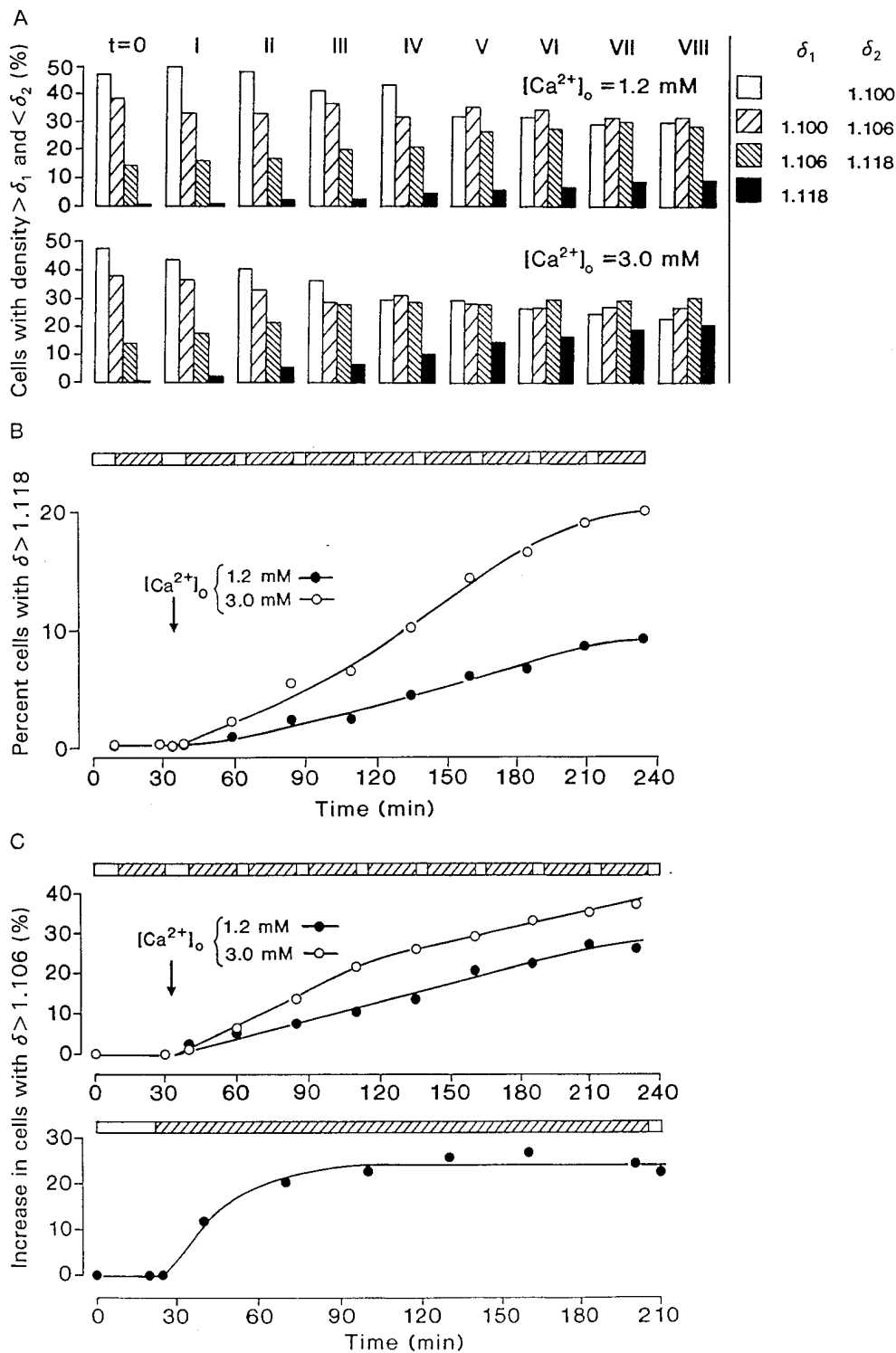
Figure 6. Effects of deoxy-oxy cycling and continuous deoxygenation on the density distribution of SS discocytes. In A and B , cells suspended at 18% Hct in solution B with adenine and inosine were tonometered at 37°C, alternating deoxy (20 min) and oxy (5 min) for 4 h. After a first cycle in Ca 2+ -free media, either 1.2 or 3.0 mM CaCl 2 was added. A shows the density shifts in samples taken after each cycle and spun over the discontinuous arabinogalactan layers noted. The percentage of cells with \delta > 1.118 after each oxy-deoxy cycle and with the two [Ca 2+ ] o levels is shown in B . In C , the proportion of cells with densities increased to \delta > 1.106 after a single long deoxy pulse ( bottom panel ) is compared with that induced over time by the frequent deoxy pulsing protocol of B ( top panel ). The cells in the bottom panel are from the same experiment as those of Fig. 2 A .
