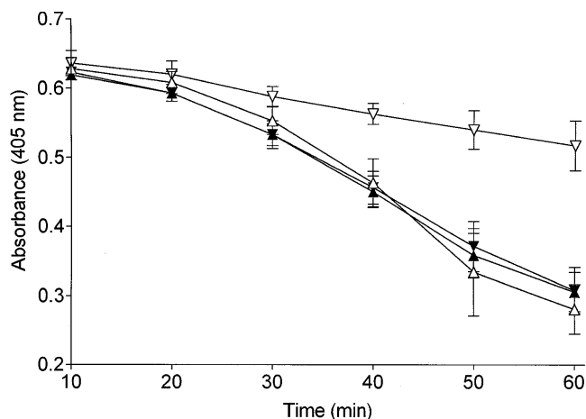
Figure 1. Lysis of a thrombin-induced clot in the presence or absence of antibodies against Factor XI or TAFI. Normal plasma was preincubated with XI-1 ( \Delta , 160 nM), mAbTAFI#16 ( \nabla , 160 nM), XI-1 and mAbTAFI#16 ( \blacktriangle , 160 nM), or buffer ( \nabla ). Coagulation was initiated by adding calcium necessary for recalcification, thrombin (20 nM), and t-PA (30 U/ml). Fibrin formation and lysis were measured in time as the change in turbidity at 405 nm. The means \pm SD of three independent experiments are given.
