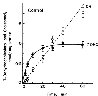
Figure 3. Conversion of [ 3\alpha - ^3\text{H} ]lathosterol to 7-dehydrocholesterol (7DHC) and cholesterol (CH) by control microsomes. Each point represents the mean \pm SD for seven subjects. 7-Dehydrocholesterol was produced rapidly after the reaction was started, and its mass increased linearly over 5 min. Cholesterol was not formed abundantly until after 10
