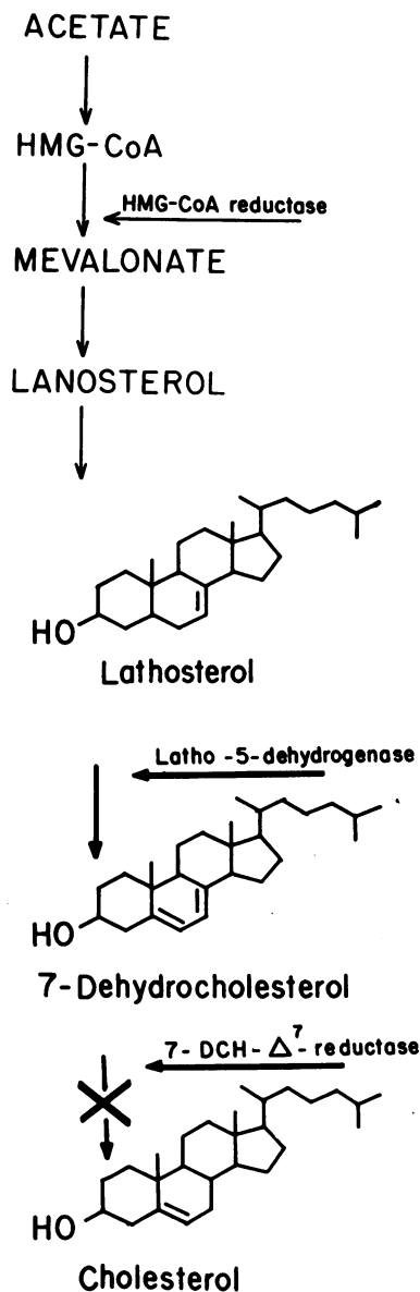
Figure 1. Flow diagram showing key intermediates in the pathway for the formation of cholesterol from acetate. HMG-CoA reductase is considered the rate-controlling enzyme that regulates the formation of mevalonic acid, the first almost totally committed precursor in the pathway. Lanosterol the first cyclized sterol is also noted. Two key reactions in late cholesterol biosynthesis are emphasized: the conversion of lathosterol to 7-dehydrocholesterol catalyzed by lathosterol-5-dehydrogenase, and the transformation of 7-dehydrocholesterol to cholesterol catalyzed by 7-dehydrocholesterol- \Delta^7 -reductase. The suspected abnormal reaction between 7-dehydrocholesterol and cholesterol in the Smith-Lemli-Opitz syndrome is denoted by a cross.
