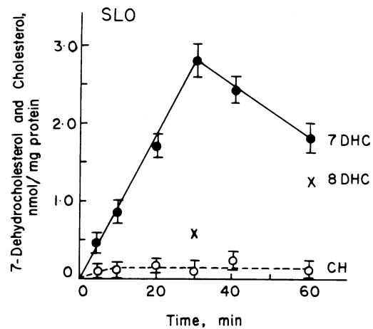
Figure 4. Conversion of [ 3\alpha - ^3\text{H} ]lathosterol to 7-dehydrocholesterol (7DHC) and cholesterol (CH) by Smith-Lemli-Opitz liver microsomes. Mean ± SD are presented for four subjects. 7-Dehydrocholesterol was produced abundantly over 30 min while virtually no cholesterol was formed. A small quantity of 8-dehydrocholesterol (8DHC) first appeared at 30 min with increased amounts at 60 min.
