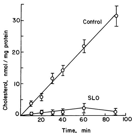
Figure 5. Conversion of [1,2- ^3\text{H} ]7-dehydrocholesterol to cholesterol by control ( n = 7 ) and Smith-Lemli-Opitz ( n = 4 ) liver microsomes. Mean \pm SD are plotted. Cholesterol was produced linearly over 90 min in the control incubations while little cholesterol was formed from 7-dehydrocholesterol by the Smith-Lemli-Opitz microsomes.
