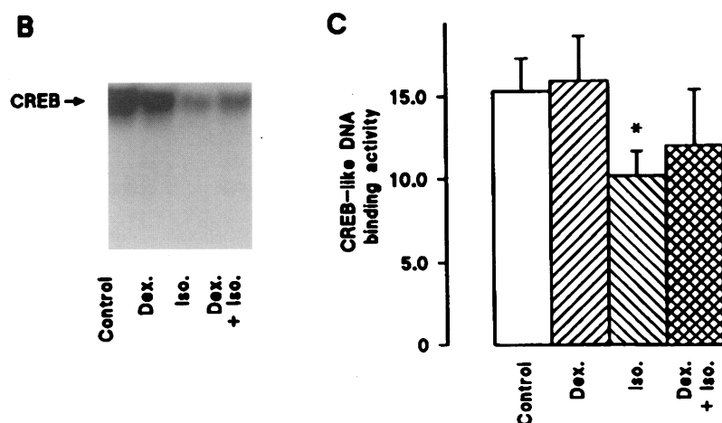
Figure 5. Effects of treatment with Dex and/or Iso on CREB-like DNA-binding activity in rat lung. (A) Specificity of the nuclear protein-CREB consensus oligonucleotide complex. The indicated amounts of nuclear protein from one control animal were incubated with the indicated amounts of ^{32}\text{P} -labeled CREB consensus oligonucleotide in the presence or absence of unlabeled competitor oligonucleotide. Arrow indicates the specific complex. (B) Representative autoradiogram from gel shift assay of CREB in rat lung. Nuclear protein from one control, one Dex-treated, one Iso-treated, and one Dex and Iso-treated rat lung was hybridized with a ^{32}\text{P} -labeled CREB consensus oligonucleotide. Arrow indicates the specific complex. (C) Densitometric measurement of CREB-like DNA-binding activity from control, Dex-treated, Iso-treated, and Dex and Iso-treated rat lungs ( n = 5 in each group). Significant different from the control value. * P < 0.05 .
