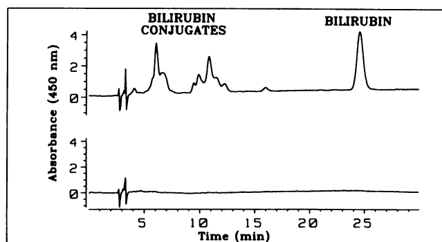
Figure 4. High-performance liquid chromatography (32) of plasma from a patient with PBC before photobleaching ( top ) and after photobleaching ( bottom ). Bleaching destroyed conjugated and unconjugated bilirubin. The bilirubin conjugates appear as broad groups of peaks because they include not only bilirubin diglucuronide, which elutes near 6 min, and the two bilirubin monoglucuronides, which elute at 11–12 min, but also numerous acyl-migration isomers of these.
