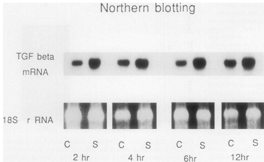
Figure 2. Induction of TGF \beta 1 mRNA expression by exposure to shear stress. Total RNA was harvested from BAEC exposed to 20 \pm 2 dynes/cm 2 and compared to static controls harvested at the same time. TGF \beta 1 mRNA expression was assessed by Northern blot ( 30 \mu\text{g}/\text{lane} ) (upper lanes). The blot was rehybridized with a 28S ribosomal RNA probe as an internal control that is unaffected by shear stress.
