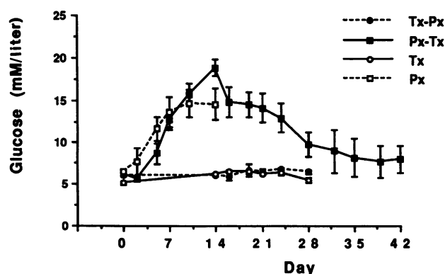
Figure 1. Evolution of fed blood glucose in experimental groups. Groups are described in Table I. Values are mean±SEM.
