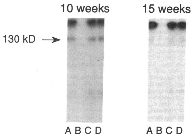
Figure 7. The effect of EGF and FGF on [ 125 I]-IGF-I binding. Placental fibroblasts (10 and 15 wk gestation) were grown to confluence. The cells were exposed to EGF (10 ng/ml) or FGF (100 ng/ml) for 4 h. [ 125 I]-IGF-I was covalently crosslinked to cell surface receptors as described and subjected to SDS-PAGE under reducing conditions. The gels were dried and exposed to x-ray film for 4 d. (A) Control binding to untreated cells. (B) Nonspecific binding in the presence of 200 ng/ml IGF-I. (C) Binding to cells treated with EGF. (D) Binding to cells treated with FGF.
