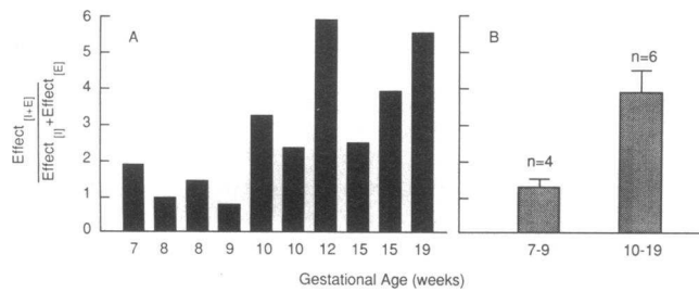
Figure 4. Potentiation of DNA synthesis by IGF-I/EGF interactions. Fibroblasts from different gestational ages were maintained in culture as previously described. Three wells were incubated with IGF-I (100 ng/ml) and EGF (10 ng/ml) alone. Three tandem wells were treated with IGF-I and EGF simultaneously. DNA synthesis resulting from the simultaneous addition of IGF-I and EGF was divided by the sum of the individual effects of IGF-I and EGF. This value is expressed as a single ratio. Purely additive effects would result in a ratio of 1 whereas synergistic effects would result in ratios > 1 . (A) Representative ratios from fibroblasts of different gestational ages. (B) Ratios shown in A were placed into two groups (7–9 wk, 10–19 wk) and averaged. The data represent the mean \pm SEM. The difference between the means of the two groups is statistically significant ( P < 0.05 ).
