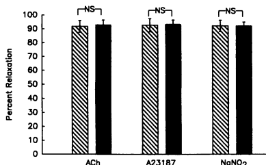
Figure 6. Summary of responses of nonischemic LCX coronary rings to 100 nM ACh, 1 \mu M A-23187, and 100 \mu M NaNO 2 . Bar heights are means, brackets indicate \pm SEM for 8–10 rings. MI + MAbR 3.1 (▨). MI + MAbR 15.7 (■).
