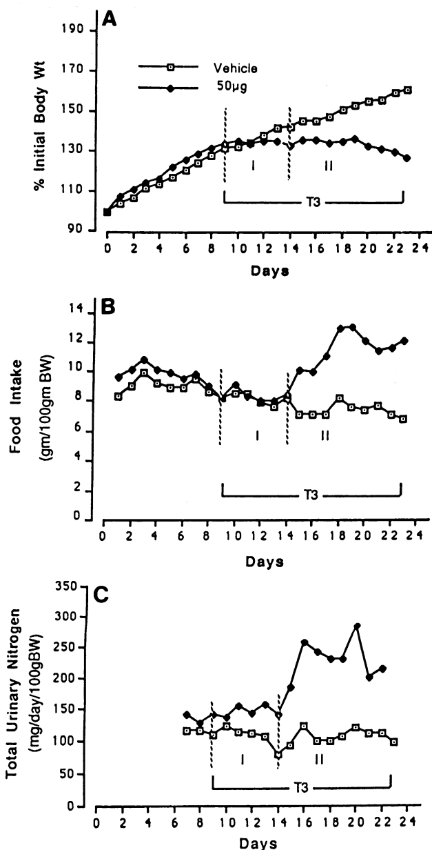
Figure 2. The effect of treatment of euthyroid rats with 50 µg T3/100 g BW on body weight (A), food intake (B), and total urinary nitrogen (C). Data are taken from Experiment 2, Table I. See legend to Fig. 1 for experimental details. Initial body weights for the T3-treated group were 193±5 g (n = 5). The control group is the same as that represented in Fig. 1.
