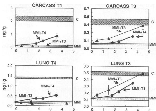
DOSES INFUSED INTO THE MOTHERS ( \mu\text{g T}_4 or \text{T}_3 / 100 g BW / day)
