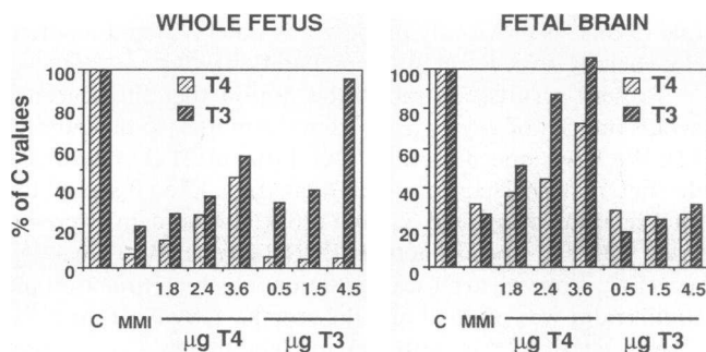
Figure 5. The left panel shows the total extrathyroidal pools of \text{T}_4 (light-hatched bars) and of \text{T}_3 (dark-hatched bars) in fetuses from C and MMI-treated dams, and from \text{T}_4 or \text{T}_3 -infused MMI-treated dams. The extrathyroidal pools corresponding to C fetuses ( 11.19 \text{ ng T}_4 and 2.42 \text{ ng T}_3 ) are taken as the 100% values. The right panel shows the amounts of \text{T}_4 and \text{T}_3 in the fetal brain. The values corresponding to C fetuses ( 0.221 \text{ ng T}_4 and 0.208 \text{ ng T}_3 ) are taken as the 100% values.
