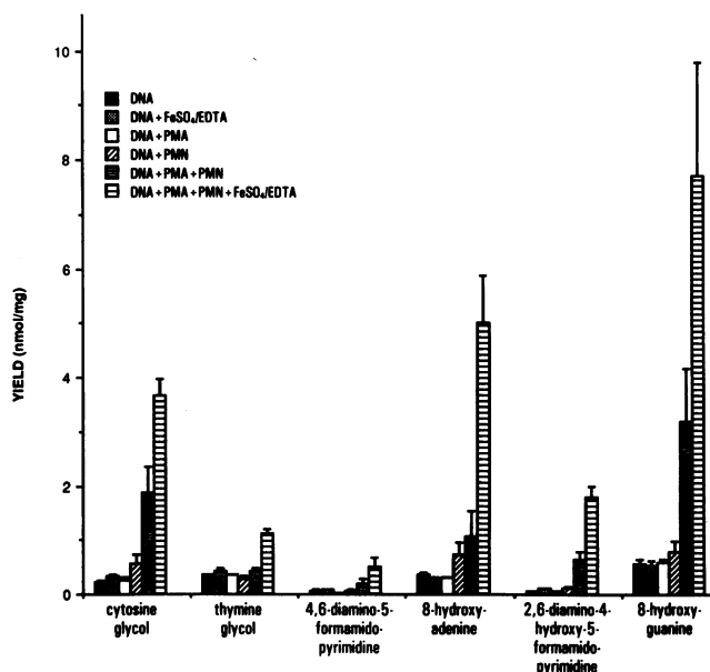
Figure 4. Yields of the base products in DNA. Reaction conditions were the same as those given in Fig. 1. Each data point represents the mean ( \pm SD) from at least three independent experiments.
