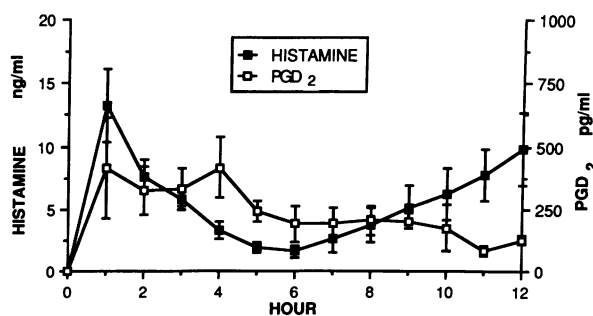
Figure 4. Time kinetics for histamine release and PGD_2 production in antigen-stimulated skin chambers. Histamine release occurs immediately after antigen challenge and can be seen to peak during the first hour. Histamine then reaches a nadir at hour 6 followed by a slow, steady increase up to hour 12. PGD_2 production peaks during the first 4 h. In contrast to the kinetics of histamine release, PGD_2 does not show an elevation during the later time periods that is consistent with the biochemical profile of the basophil.
