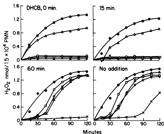
Figure 8. Contrasting effect of DHC B on the H 2 O 2 secretory response of PMN to rTNF \alpha (○) or \beta (∇) (100 ng/ml), FMLP (Δ) (5.6 × 10 -6 M), or PMA (●) (30 ng/ml). PMN were added to FBS-coated plates at time zero. DHC B (5 μg/ml) was added at the times indicated at the top of each panel. There was no effect of adding 0.17% dimethylsulfoxide (solvent for DHC B) at time zero (not shown). (×) No stimulus.
