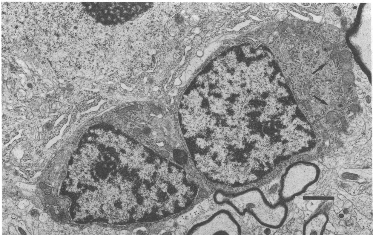
Figure 7. Two neuroglial cells in close approximation to a neuron in the cerebral cortex of another transplanted MPS I dog. The glial cell on the right has more lysosomes (arrows) than the other neuroglial cell or the neuron, but none appears to be accumulating large amounts of
