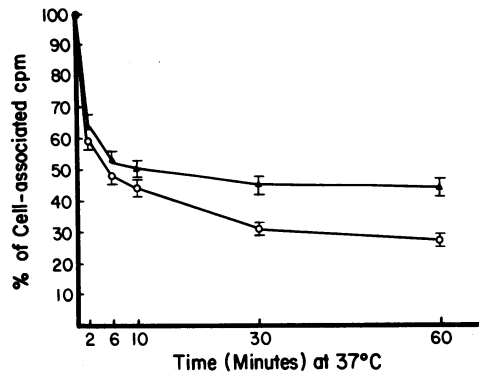
Figure 6. ^{59}\text{Fe} -Tf release from cells. HL60 cells grown for 24 h in media containing 50 \mu\text{g}/\text{ml} of Tf-Ga (○) or Tf-Zn (△) were harvested, washed, and incubated with ^{59}\text{Fe} -Tf for 4 h at 4°C to permit binding of ^{59}\text{Fe} -Tf to cell surface transferrin receptors. Unbound ^{59}\text{Fe} -Tf was removed by washing and the cells were resuspended in 200 \mu\text{l} of buffer and incubated at 37°C for 1 min, and 1 ml of warm media containing 50 \mu\text{g}/\text{ml} of Tf-Ga or Tf-Zn was then added to the corresponding cells and the incubation was continued at 37°C. Aliquots of cell suspensions were removed at 0, 2, 6, 10, 30, and 60 min after addition of warm media, rapidly cooled to 4°C, and centrifuged. Cell pellets and supernatants were then counted separately for ^{59}\text{Fe} radioactivity and the percentage of radioactivity remaining in the cells was determined. Points represent mean of three experiments \pm SD.
