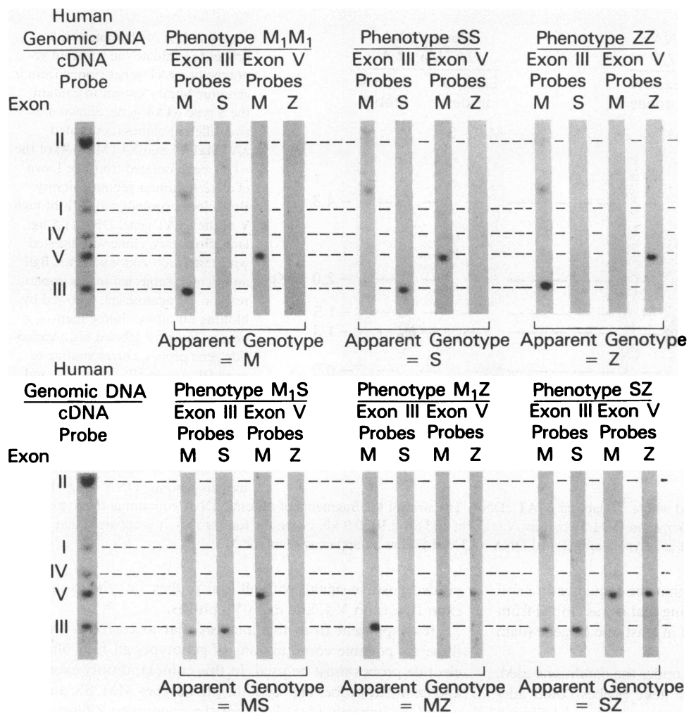
Figure 3. Use of oligonucleotide probes to correctly identify all possible combinations of M, S, and Z haplotypes. Genomic DNA (5 µg/lane) from six different individuals, representing known phenotypes M 1 M 1 , SS, ZZ, M 1 S, M 1 Z, and SZ, were digested with the endonucleases BglI and EcoRI, electrophoresed on 1% agarose gel, blotted to nitrocellulose filters, and hybridized with 32 P-labeled exon III M , exon III S , exon V M , and exon V Z probes. After being washed, the nitrocellulose strips were autoradiographed for 2 d at -70°C. As a control, at the left is shown genomic DNA cut with the same endonucleases and hybridized with 32 P-labeled cDNA, thus identifying DNA fragments containing exons I-V (see legends to Figs. 1, 2). The apparent genotype of each sample determined by oligonucleotide probe analysis is below the four electrophoretograms of each phenotype.
