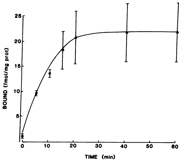
Figure 1. Specific binding of 1 nM [ ^3\text{H} ]nitrendipine to adrenal zona glomerulosa membranes obtained from rats on a normal NaCl diet. Binding was examined at pH 7.4 at 22°C (mean \pm SEM, n = 2 experiments). Nonspecific binding determined in the presence of 1 \mu\text{M} unlabeled nitrendipine, reached equilibrium by 10 min.
