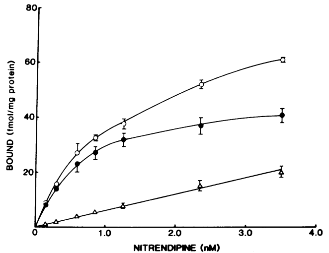
Figure 2. Equilibrium binding of [ ^3\text{H} ]nitrendipine to rat adrenal zona glomerulosa membranes obtained from rats on a normal NaCl diet. Binding was examined as described in Fig. 1 for 60 min: total binding ( \circ ), specific binding ( \bullet ), and nonspecific binding ( \Delta ) (mean \pm SEM, n = 2 experiments). The Scatchard plot of these data are presented in Fig. 3.
