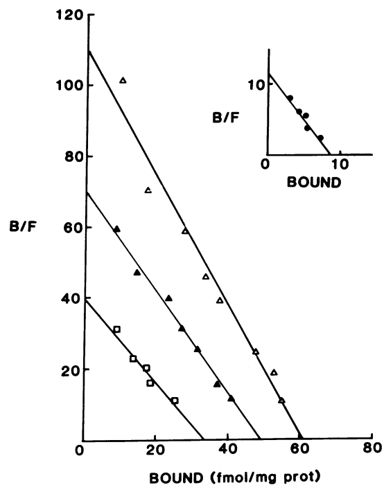
Figure 3. Representative Scatchard plots of binding data. Scatchard plot of [ ^3\text{H} ]nitrendipine binding to membranes of rat mesenteric artery ( \bullet ), aorta ( \square ), adrenal zona glomerulosa ( \blacktriangle ), and uterus ( \Delta ). Binding studies were performed as in Fig. 2. Mesenteric artery, aorta, and uterine tissues were obtained during NaCl restriction and adrenal zona glomerulosa during a normal NaCl diet.
