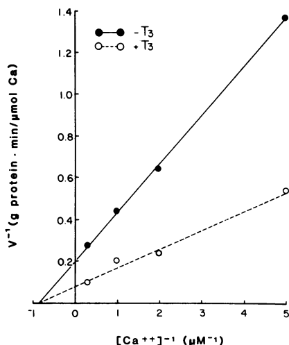
Figure 3. Calcium uptake by L6 cell crude homogenates. Data are analyzed by Lineweaver-Burk plots. Half the cells were maintained in serum free media without T3 and half with T3 for 3 d before harvesting. Analysis indicates the K_m is identical for both homogenates (1.2 \mu\text{M} ), but the V_{\text{max}} is 2.5-fold greater in the T3-treated homogenates (12.8 vs. 5 \mu\text{mol Ca/g} protein per min). Total protein per petri dish was 1.0 mg in the absence of T3 and 0.9 mg in the presence of T3.
