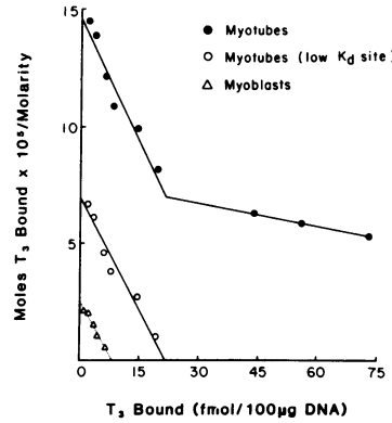
Figure 1. Scatchard analysis of T3 binding to receptors in nuclear preparations of L6 myotubes and undifferentiated myoblasts. The myotube data are replotted to show only the binding to the high affinity site, by extrapolation of the low affinity binding site portion of the curve and subtraction of this line from the high affinity sites from myotubes and myoblasts have identical slopes, indicating that
