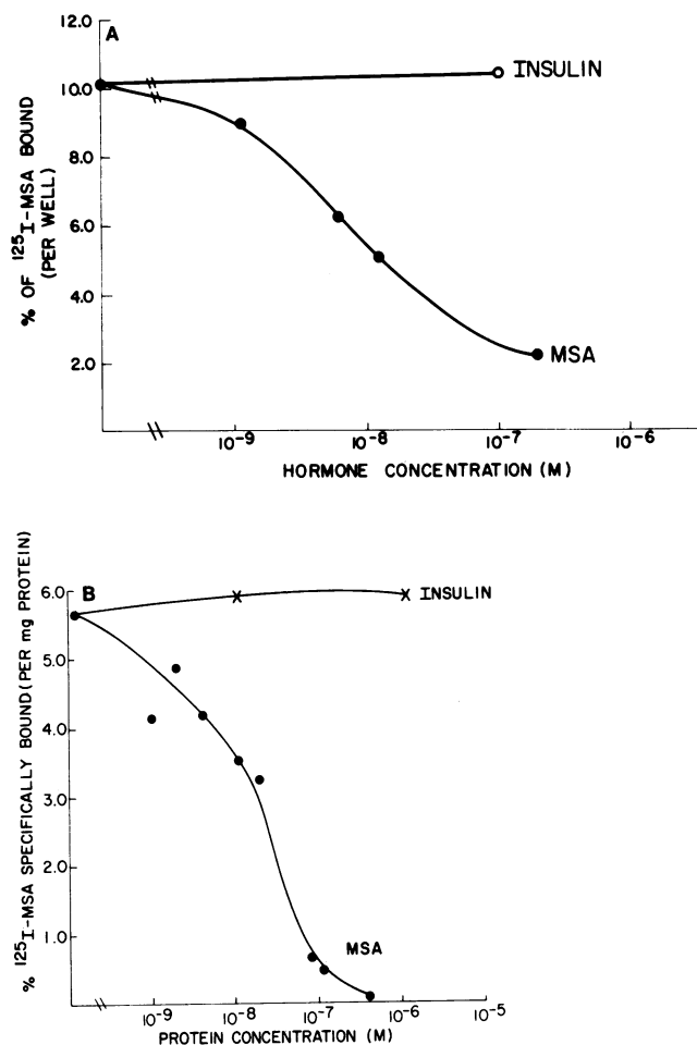
Figure 5. Inhibition of ^{125}\text{I} -MSA binding to (A) aortic smooth muscle cells and (B) retinal capillary pericytes by unlabeled MSA and insulin. The data shown are for one of two similar experiments. Each point is the average of duplicates in one experiment.
