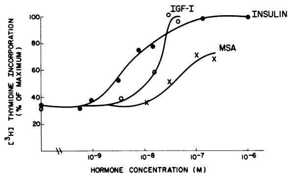
Figure 6. Effect of insulin (●), IGF-I (○), and MSA (×) on ^3\text{H} thymidine incorporation into DNA of retinal capillary endothelial cells. Each point is the average of triplicate wells in each experiment. Almost confluent cultures were exposed to these growth factors for 16–20 h at 37^\circ\text{C} and then labeled with ^3\text{H} thymidine for 30 min. Detailed description of the insulin study was reported earlier (7).
