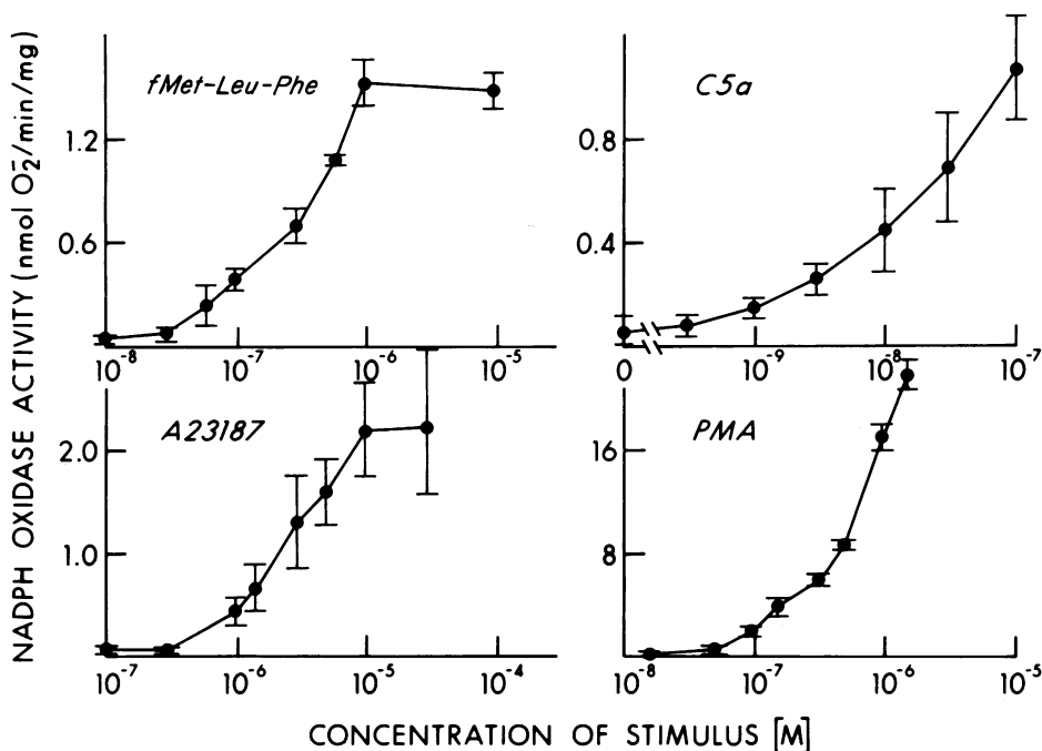
FIGURE 2 NADPH oxidase activity as a function of stimulus concentration. PMN were exposed to various concentrations of either fMet-Leu-Phe for 1 min, C5a for 30 s, A23187 for 5 min, or PMA for 15 min in the presence of CB. Particulate fractions were then isolated and assayed. Data are expressed as the mean±SEM of two to five experiments with each dose of stimulus.
