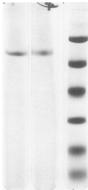
FIGURE 2 SDS-PAGE of normal and patient M.F.'s prothrombin. Left, normal prothrombin without, and with prior treatment with \beta -mercaptoethanol and markers. Right, patient without and with \beta -mercaptoethanol and markers as for normal prothrombin previously. In both sets the top two marker bands are 94,000 and 67,000 daltons, respectively. Normal prothrombin contained 9.5 units antigenic prothrombin/mg, 7.2 units prothrombin activity/milligram with activity/antigen ratio 0.76. Patient prothrombin contained 8.8 units antigenic prothrombin/milligram, 2.4 units prothrombin activity/mg with activity/antigen ratio 0.27.
