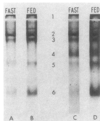
FIGURE 2 The Coomassie Blue-stained SDS 10% polyacrylamide gel electrophoresis of apoproteins on the recovered emulsion from a 30-min fasted (A) and fed (B) liver in studies where the original emulsion was not enriched in E apoproteins. The apoprotein pattern of the recovered emulsion from studies where the initial emulsion was supplemented with apoprotein E; lane C from a fasted hepatic perfusion and lane D from a fed. Band 1 represents undefined protein aggregates at the site of gel entry; 2 is serum albumin; 3 a partially characterized basic protein; 4 is apo E; 5 is an uncharacterized apoprotein; 6 is apo CII and CIII proteins.
