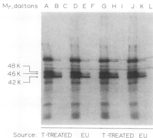
FIGURE 6 Cholera toxin-catalyzed [ ^{32}\text{P} ]ADP-ribosylation of proteins of hepatocyte homogenates from control as compared with hyperthyroid rats. Hepatocytes were isolated from control animals or animals administered 25 \mu\text{g} of triiodothyronine/100 g body wt at 48, 24, and 3 h prior to cell isolation. Whole homogenate fractions were prepared and cholera toxin catalyzed ADP-ribosylation was performed using [ ^{32}\text{P} ]NAD ^{+} . The details of the intoxication, SDS-polyacrylamide gel electrophoresis, and autoradiography appear in the legend to Fig. 4. Equivalent amounts of homogenate protein were used and the amount of protein loaded onto the gels was 0.1 mg in all lanes. Hepatocyte homogenates obtained from T_3 -treated (lanes A-C, G-I), and control (lanes D-F, J-L) rats were treated with no toxin (lanes C, F, I, L), 5.0 \mu\text{g}/\text{ml} of activated toxin (lanes B, E, H, K), or 50 \mu\text{g}/\text{ml} of activated toxin (lanes A, D, G, J). This autoradiogram is representative of three such experiments, each performed with different rat hepatocyte membrane preparations.
