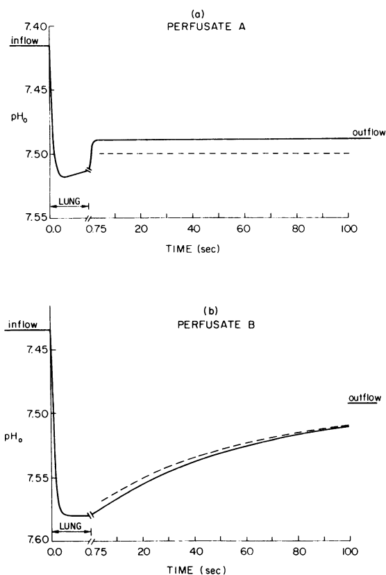
FIGURE 4 Predicted (solid curves) and actual (dashed curves) time-courses of perfusate extracellular pH during and after capillary transit for lung 1, pair b. The upper panel shows pH_0 vs. time for perfusate A, while the lower panel shows pH_0 vs. time for perfusate B. Inflowing perfusate blood gas values used in computing the time-courses were: pH_0 = 7.416 , PCO_2 = 33.0 torr, and PO_2 = 43.4 torr for perfusate A; and, pH_0 = 7.434 , PCO_2 = 31.7 torr, and PO_2 = 42.7 torr for perfusate B. Alveolar gas tensions used were PCO_2 = 25.5 torr and PO_2 = 110 torr for perfusate A, and PCO_2 = 22.5 torr and PO_2 = 103 torr for perfusate B. Extracellular buffer capacity was 1.4 \text{ mM H}^+/\text{pH} for perfusate A and 0.92 \text{ mM H}^+/\text{pH} for perfusate B. Extracellular catalyzing factors used in these computations were 100 for both perfusate B and perfusate A. Intracellular catalyzing factor was taken as 6,500 in both perfusates. Bicarbonate and chloride permeability of the RBC membrane was 6.0 \text{ nm/s} for perfusate B, and 1 \text{ } \mu\text{m/s} for perfusate A. Other parameter values used in these computations have been given previously (18).
