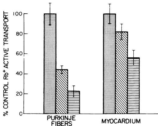
FIGURE 3 Comparison of Rb + active transport in Purkinje fibers and myocardium from animals not exposed to digoxin ( n = 8; stippled bars), chronically dosed animals receiving 0.02 mg/kg digoxin daily ( n = 8; diagonally hatched bars), and animals at onset of ventricular tachycardia after acute administration of 0.3 mg/kg digoxin ( n = 8; horizontally hatched bars). Values are reported as percentage change compared to active transport in animals not receiving digoxin. The percent inhibition is significantly greater in the Purkinje fibers than in the myocardium for both acute and chronic dosage regimens ( P < 0.01).
