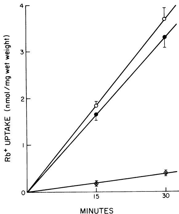
FIGURE 1 Time-course of Rb^+ uptake by canine Purkinje fibers in vitro . Values are mean \pm SEM. 10 Purkinje fibers (2–8 mg wet wt) were studied at each time point, half of which were incubated in the presence of 0.1 mM Rb^+ including tracer ^{86}Rb^+ and the other half with both Rb^+ and 1 \mu M ouabain. Upper curve (○) shows total Rb^+ uptake in the absence of ouabain; the lower curve (○) shows uptake in the presence of 1 \mu M ouabain. The difference is plotted (●) as active Rb^+ transport.
