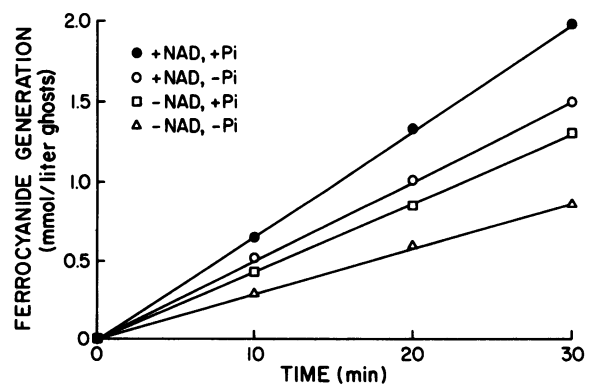
FIGURE 6 The effect of the omission of NAD and/or Pi on the rate of ferrocyanide generation by resealed ghost preparations containing all other components of the NADH generating system. (DHA concentration 50 \mu M).
