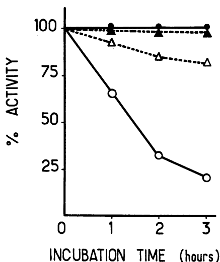
FIGURE 6 Heat stability of MPG as a function of time in crude 1/15 hemolysates from the propositus (—○—) and from control (—△—) and after addition of 5 mM 2,3-DPG in hemolysates from the propositus (—●—) and from control (—▲—). Incubation was performed at 50°C. The noncentrifuged hemolysates contained 0.7 mM \beta -mercaptoethanol and 1 mM EDTA. Results are expressed as a percentage of the MPG activity of each nonincubated hemolysate.
