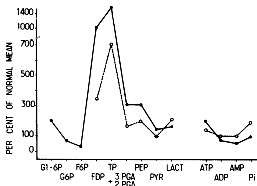
FIGURE 2 Crossover plot of the concentration of glycolytic intermediates in the erythrocytes from the propositus (—●—) and from his son (---○---). The glycolytic compounds were determined after deproteinization in neutralized acid extracts on fresh heparinized blood. Results are expressed for each intermediate as a percentage of the normal mean calculated from 10 controls. PEP denotes phospho-enol-pyruvate; Pi denotes inorganic phosphates; PYR represents pyruvate; LACT denotes lactate.
