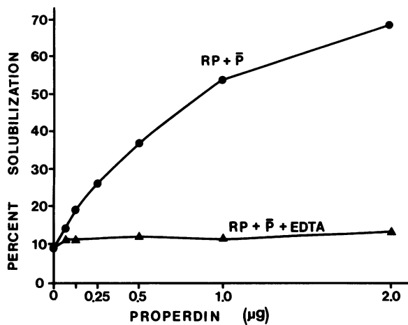
FIGURE 1 Reconstitution of CRA by RP and pure \bar{P} . Various amounts of pure \bar{P} were added to 0.2 ml of a 1:2 dilution of RP. After the mixtures were prewarmed at 37°C for 10 min, immune precipitates of ^{125}\text{I} -BSA and anti-BSA containing 0.5 \mu\text{g} of Ab were added. Tubes were incubated for another 60 min at 37°C, then diluted with 0.4 ml of cold EDTA-GPB, and centrifuged. Supernates and pellets were assayed for radioactivity. The controls contained RP, \bar{P} , and 0.01 M EDTA.
