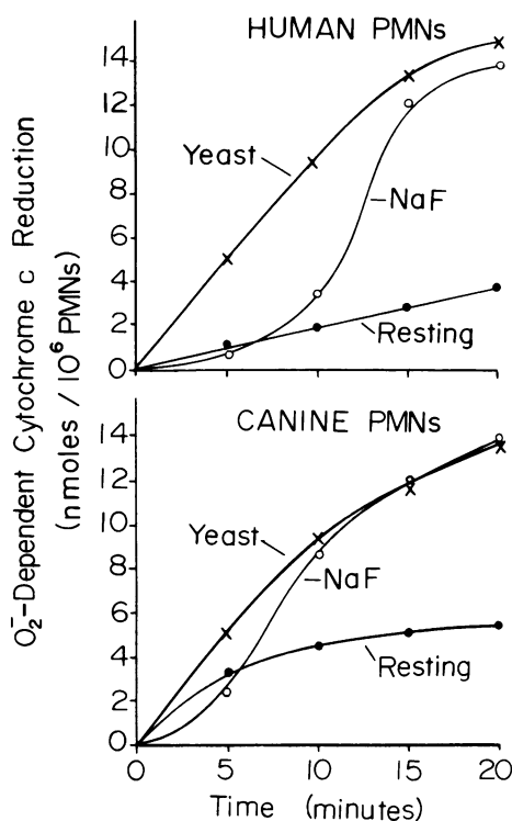
FIGURE 4 \text{O}_2^- production of resting, phagocytic, and 20 mM NaF-treated human and canine PMNs at 37^\circ\text{C} . SOD-inhibitable cytochrome c reduction was used to quantitate \text{O}_2^- produced by 1 \times 10^6 PMNs in the presence of 0.1 mM cytochrome c in HBSS. Unstimulated or resting PMNs ( \bullet ) were compared with cells treated with 20 mM NaF ( \circ ) and with PMNs mixed with 5 \times 10^7 opsonized yeast ( \times ). Data are the means of three different human and canine donors.
