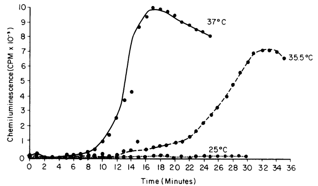
FIGURE 2 Effect of temperature on CL response of PMNs to 20 mM NaF. 5 \times 10^6 PMNs from the same donor were assayed at 37°C (—), 35.5°C (---), and 25°C (···). Base-line CL value of PMNs was 4,300 cpm.
