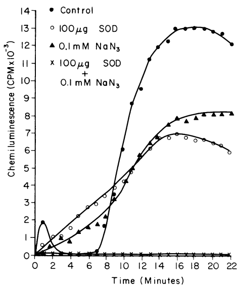
FIGURE 3 Effect of SOD and sodium azide ( \text{NaN}_3 ) on CL response of PMNs treated with NaF at 37^\circ\text{C} . Control CL response of 5 \times 10^6 PMNs in 20 mM NaF ( \bullet ) was compared with autologous PMNs treated with 20 mM NaF and 100 \mu\text{g} SOD ( \circ ); 0.1 mM \text{NaN}_3 ( \blacktriangle ); a combination of 100 \mu\text{g} SOD and 0.1 mM \text{NaN}_3 ( \times ). Protein solutions containing 100 \mu\text{g} of bovine serum albumin were similar to control CL responses.
