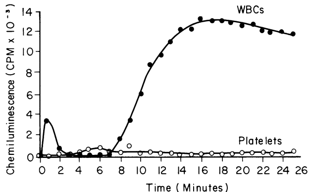
FIGURE 1 CL response of 20 mM NaF-treated leukocytes and platelets procured by a continuous flow blood cell separator. The platelet preparation (○) contained 2 \times 10^6 platelets/vial and was free of leukocytes; the leukocytes preparation (●) contained 85% PMNs and 15% mononuclear cells in a concentration of 5 \times 10^6 PMNs/vial. PMNs had a base-line CL value of 4,600 cpm and platelet CL base-line value was 2,800 cpm. WBCs, leukocytes.
