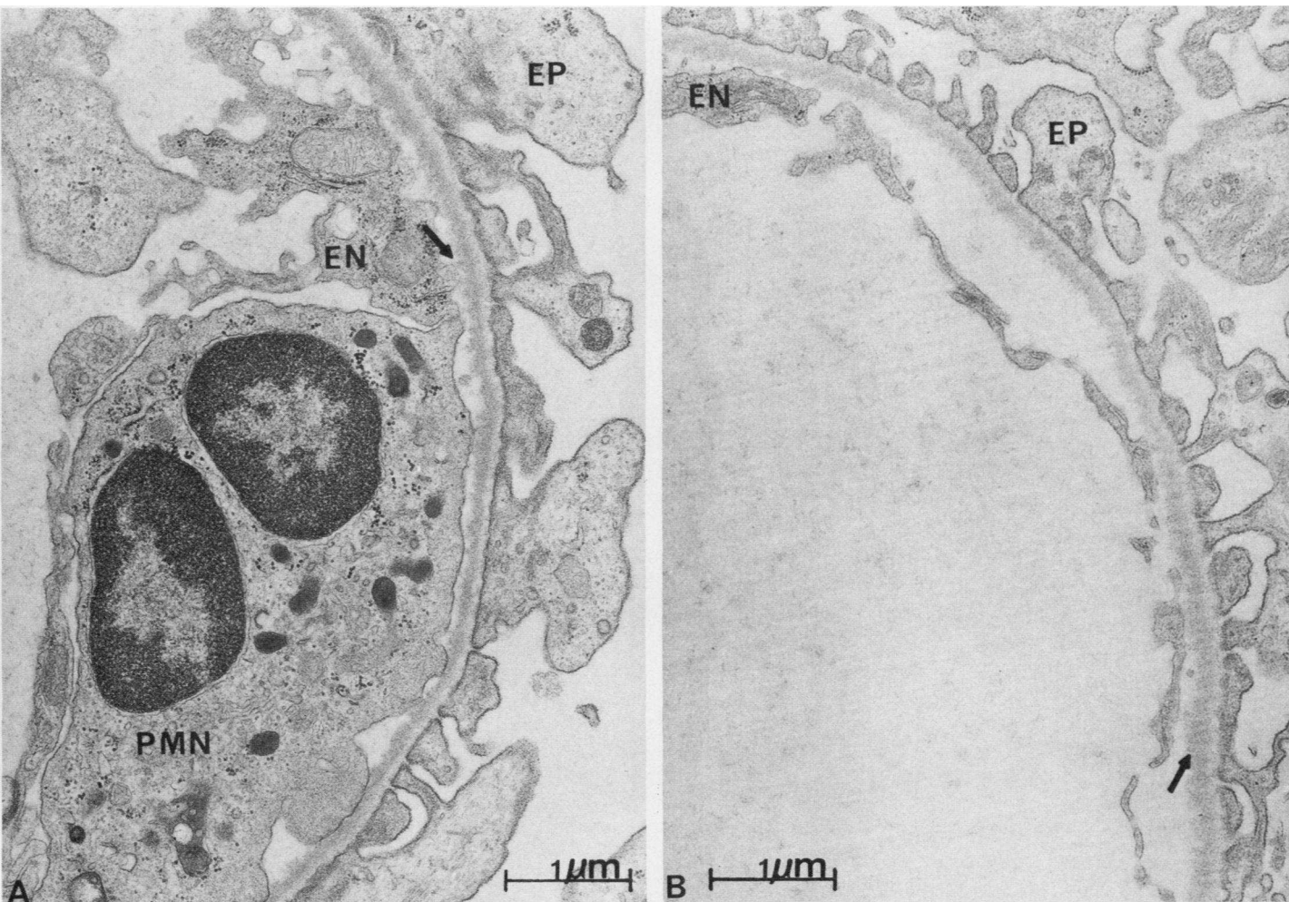
FIGURE 3 Electron microscope studies of a high-dose normal complementemic rat (A) and a complement-depleted C566-treated rat (B) are shown. The subendothelial aspect of the GBM (arrows) appeared irregular, presumably representing the fixation of anti-GBM antibody. A PMN was found approximated along the GBM displacing the endothelium (EN) in the normal complementemic rat in A. Endothelial separation occurred in the complement-depleted rat seen in B; however, PMN infiltration was almost completely lacking. Focal areas of epithelial cell (EP) foot process fusion were found and were particularly evident in A. ( \times 17,750 .)
