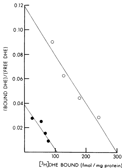
FIGURE 1 Scatchard analysis of [ 3 H]DHE binding in estrogen- and progesterone-primed uteri. Six rabbits were injected with estrogen alone (O) (estrogen-primed) by protocol II and six weight-matched rabbits were injected with estrogen followed by progesterone (●) (progesterone-primed). [ 3 H]DHE binding was determined as the mean of duplicate determinations over a range of [ 3 H]DHE concentrations from 5 to 60 nM and the data were analyzed by the method of Scatchard (12). Lines were determined by linear regression analysis ( r = 0.97 for progesterone-primed and 0.92 for estrogen-primed).
